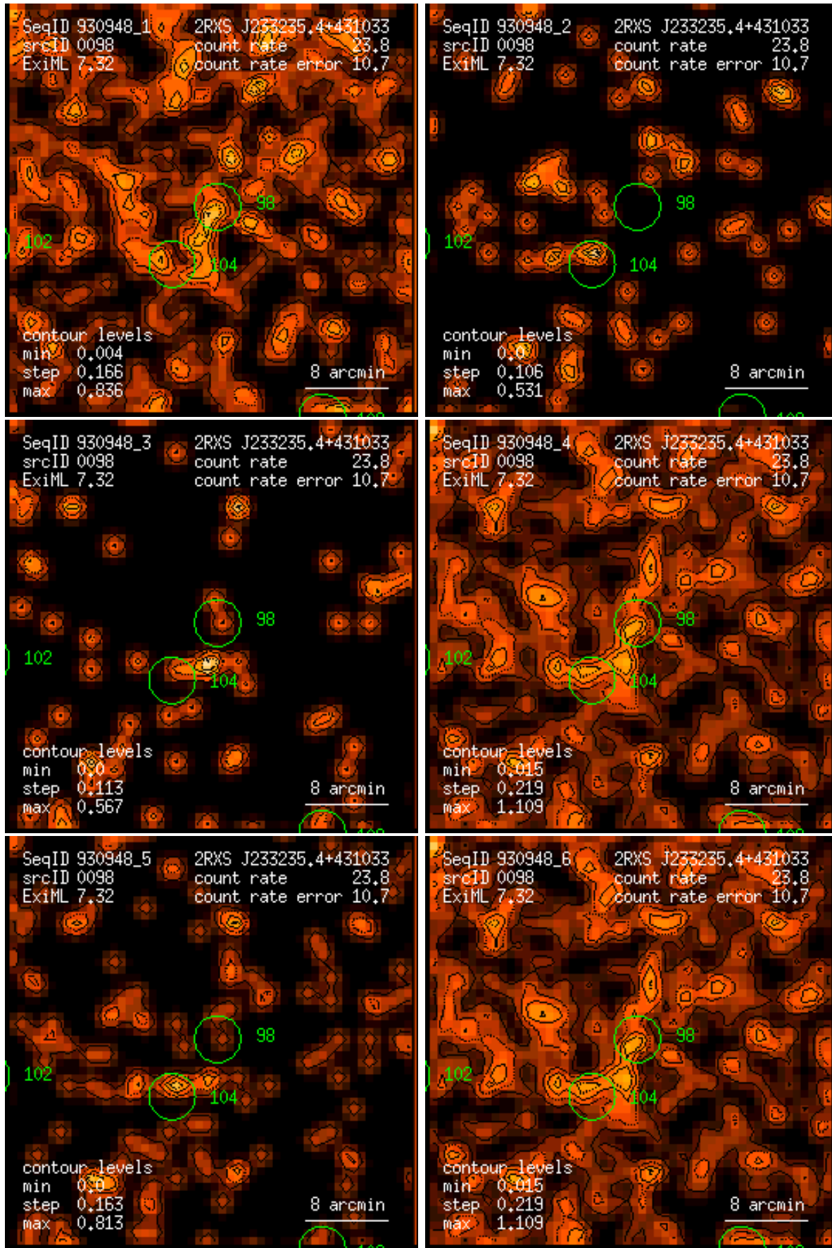
Figure 98: RASS 930948: detection 0098: band rate images, Gaussian filter: (1) PSPC channels 11 – 41, (2) 52 – 90, (3) 91 – 201, (4) 11 – 235, (5) 52 – 201, (6) 11 – 201. Broad band rates in counts/ks. Band rate contour levels in counts/ks/arcmin 2 .
