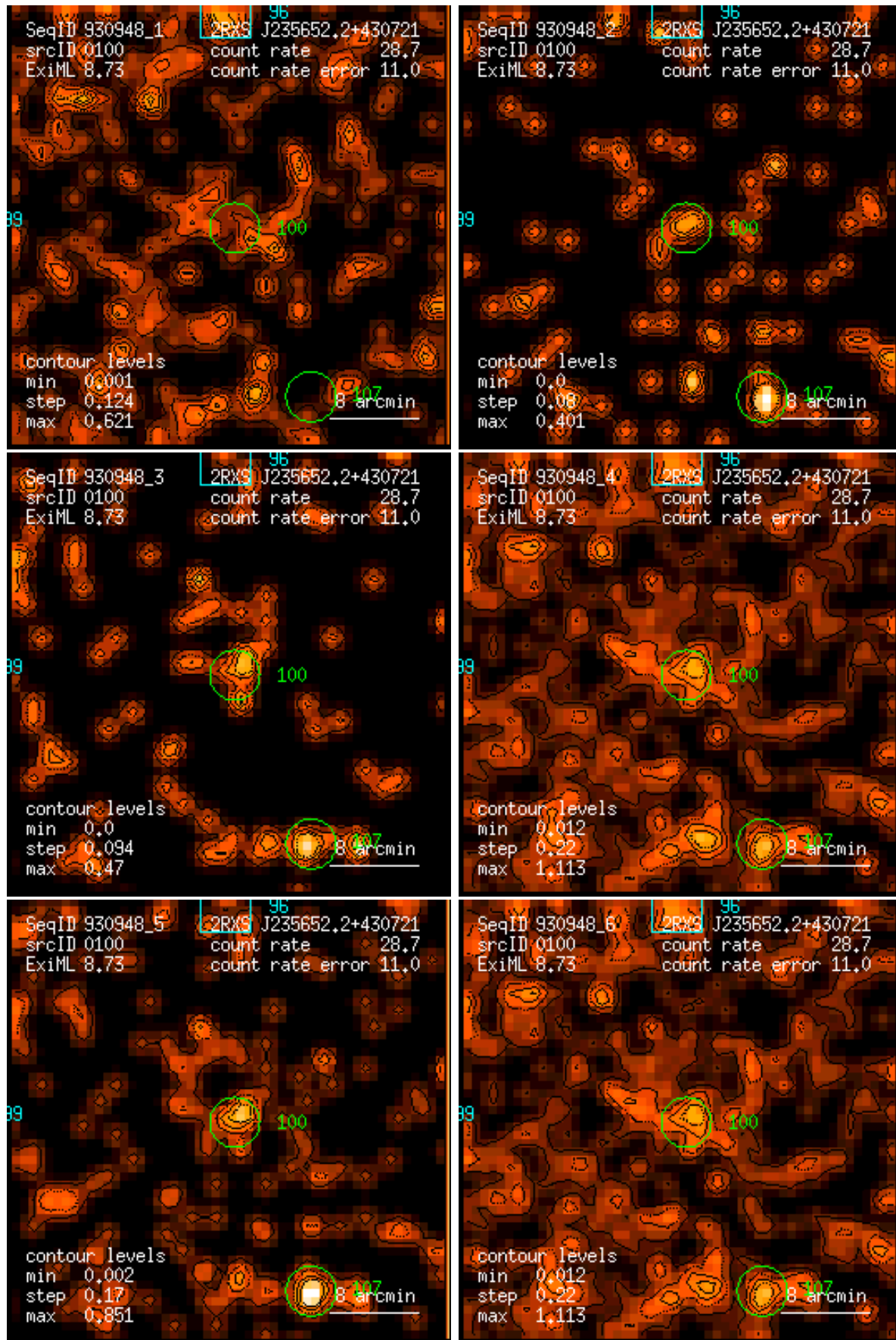
Figure 100: RASS 930948: detection 0100: band rate images, Gaussian filter: (1) PSPC channels 11 – 41, (2) 52 – 90, (3) 91 – 201, (4) 11 – 235, (5) 52 – 201, (6) 11 – 201. Broad band rates in counts/ks. Band rate contour levels in counts/ks/arcmin 2 .
