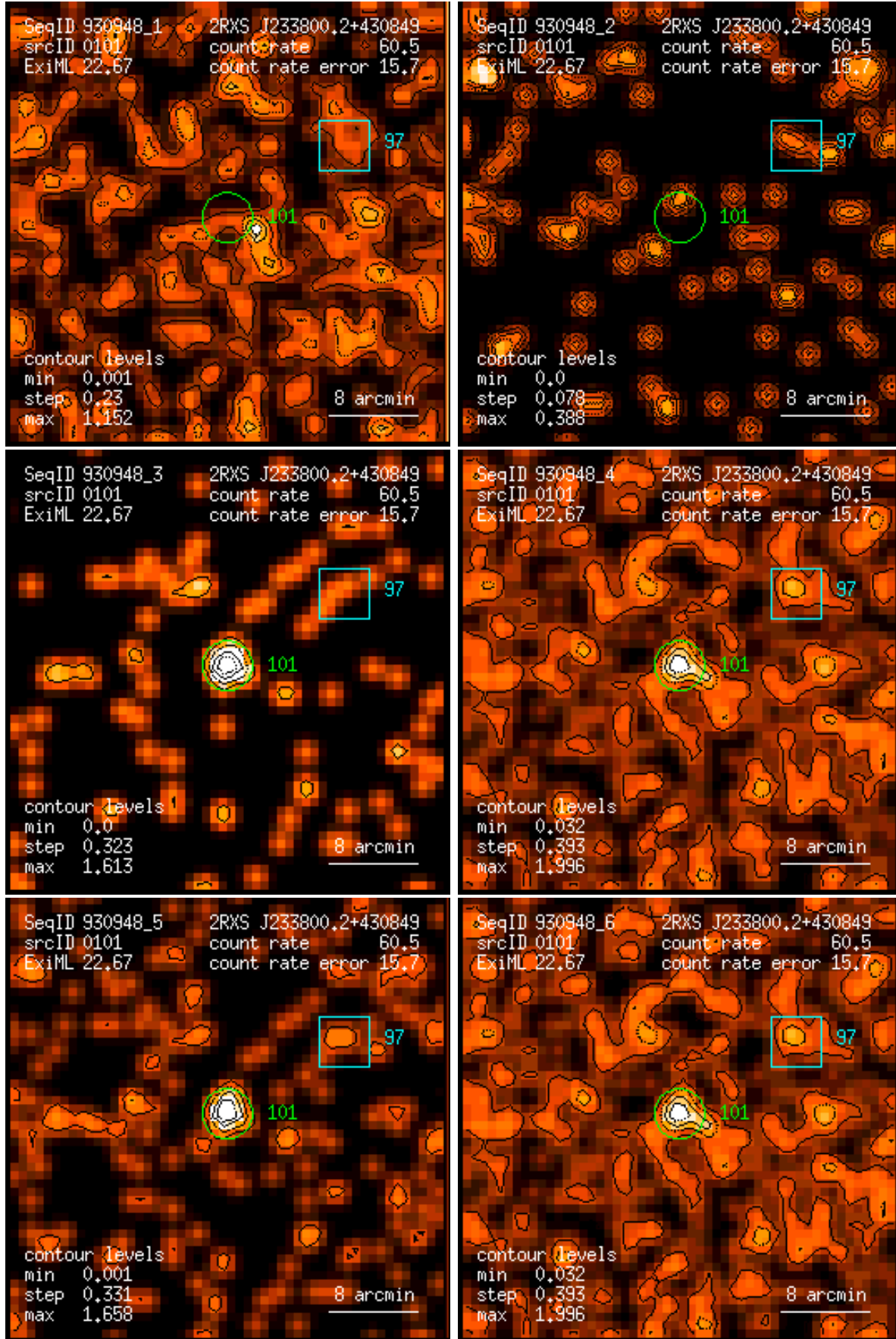
Figure 101: RASS 930948: detection 0101: band rate images, Gaussian filter: (1) PSPC channels 11 – 41, (2) 52 – 90, (3) 91 – 201, (4) 11 – 235, (5) 52 – 201, (6) 11 – 201. Broad band rates in counts/ks. Band rate contour levels in counts/ks/arcmin 2 .
