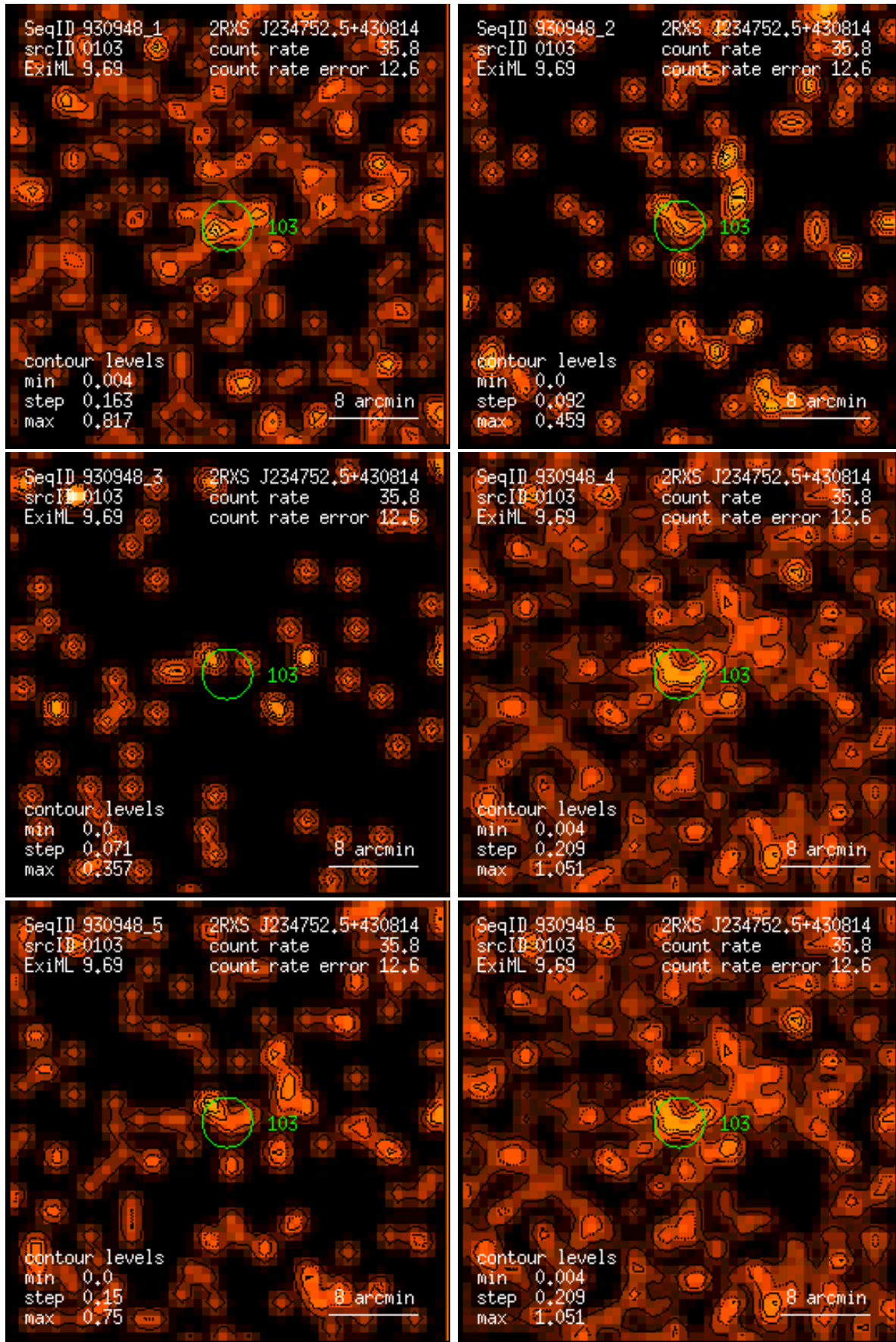
Figure 103: RASS 930948: detection 0103: band rate images, Gaussian filter: (1) PSPC channels 11 – 41, (2) 52 – 90, (3) 91 – 201, (4) 11 – 235, (5) 52 – 201, (6) 11 – 201. Broad band rates in counts/ks. Band rate contour levels in counts/ks/arcmin 2 .
