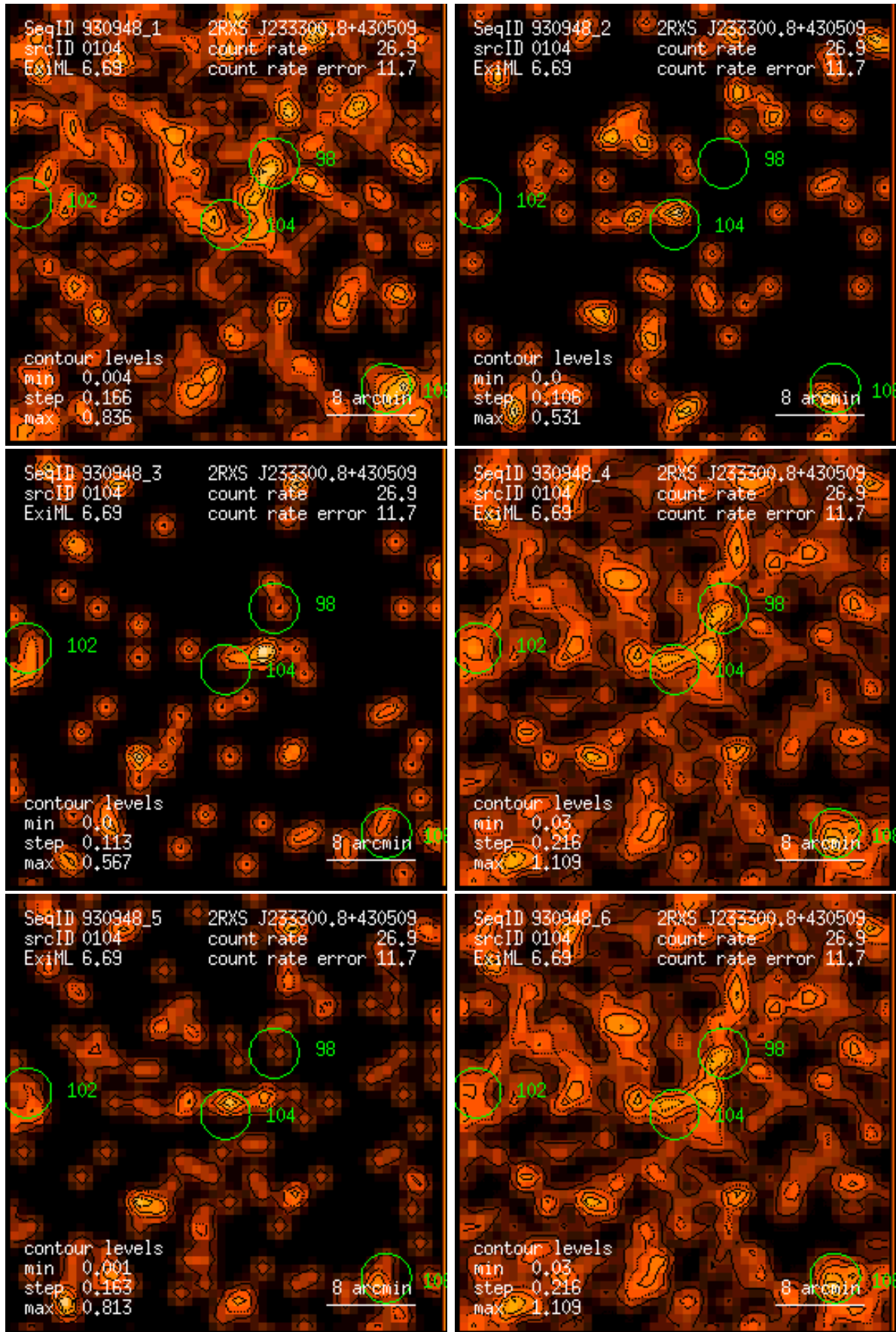
Figure 104: RASS 930948: detection 0104: band rate images, Gaussian filter: (1) PSPC channels 11 – 41, (2) 52 – 90, (3) 91 – 201, (4) 11 – 235, (5) 52 – 201, (6) 11 – 201. Broad band rates in counts/ks. Band rate contour levels in counts/ks/arcmin 2 .
