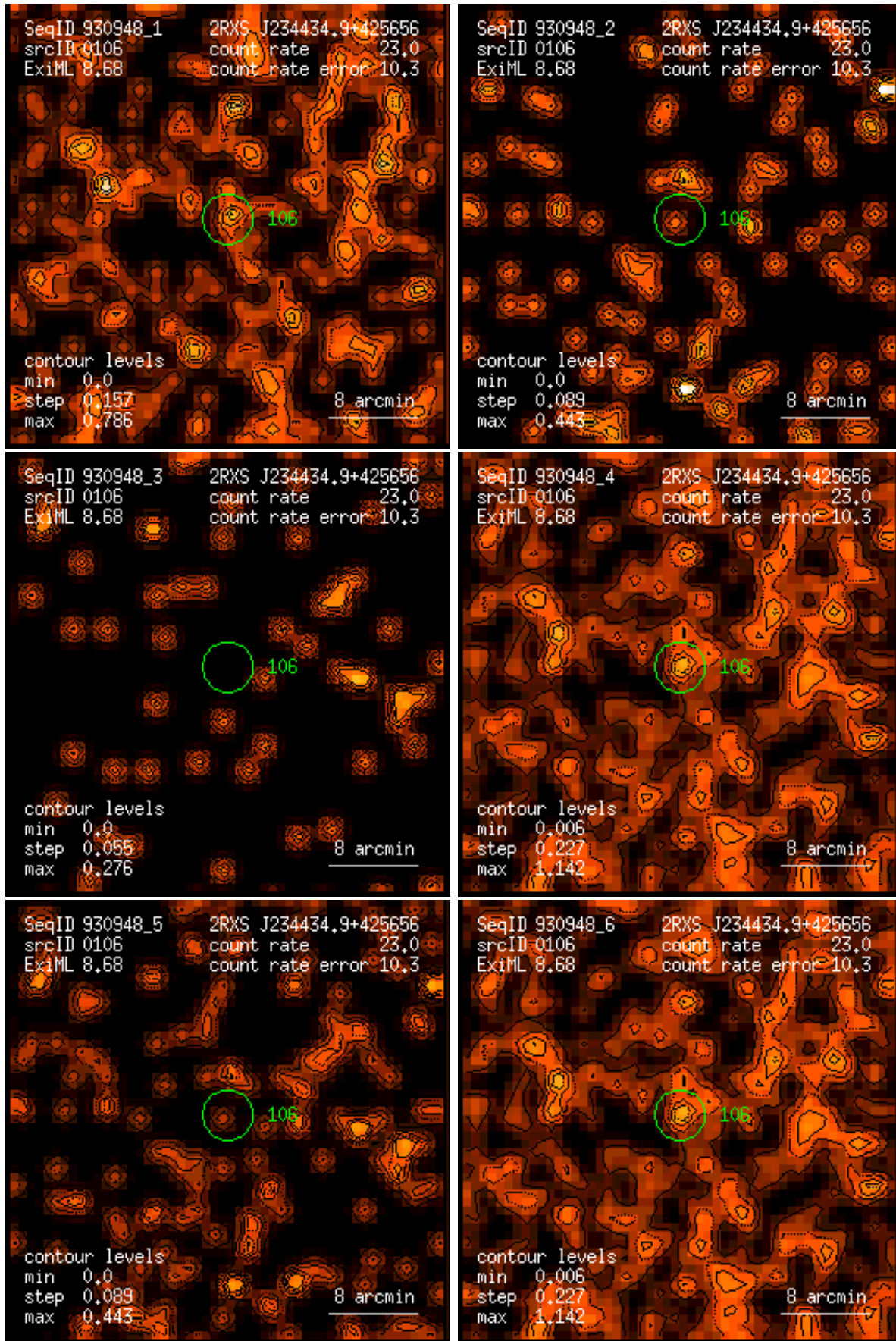
Figure 106: RASS 930948: detection 0106: band rate images, Gaussian filter: (1) PSPC channels 11 – 41, (2) 52 – 90, (3) 91 – 201, (4) 11 – 235, (5) 52 – 201, (6) 11 – 201. Broad band rates in counts/ks. Band rate contour levels in counts/ks/arcmin 2 .
