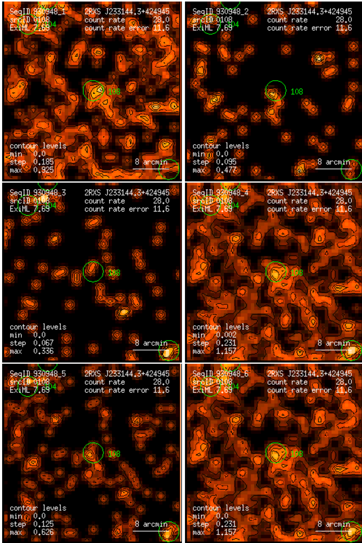
Figure 108: RASS 930948: detection 0108: band rate images, Gaussian filter: (1) PSPC channels 11 – 41, (2) 52 – 90, (3) 91 – 201, (4) 11 – 235, (5) 52 – 201, (6) 11 – 201. Broad band rates in counts/ks. Band rate contour levels in counts/ks/arcmin 2 .
