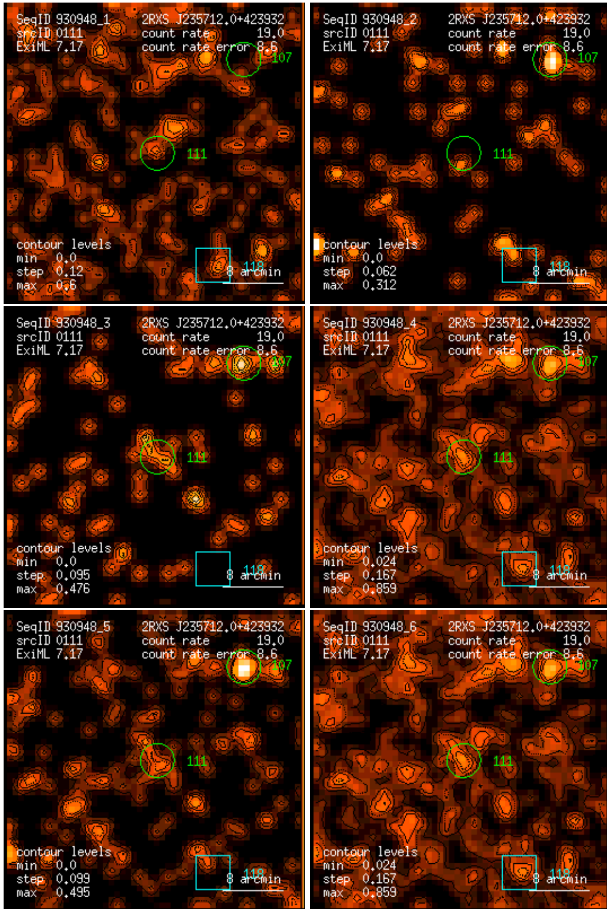
Figure 111: RASS 930948: detection 0111: band rate images, Gaussian filter: (1) PSPC channels 11 – 41, (2) 52 – 90, (3) 91 – 201, (4) 11 – 235, (5) 52 – 201, (6) 11 – 201. Broad band rates in counts/ks. Band rate contour levels in counts/ks/arcmin 2 .
