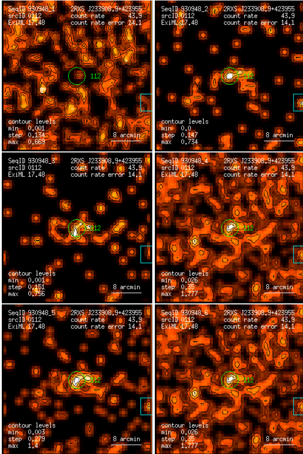
Figure 112: RASS 930948: detection 0112: band rate images, Gaussian filter: (1) PSPC channels 11 – 41, (2) 52 – 90, (3) 91 – 201, (4) 11 – 235, (5) 52 – 201, (6) 11 – 201. Broad band rates in counts/ks. Band rate contour levels in counts/ks/arcmin 2 .
