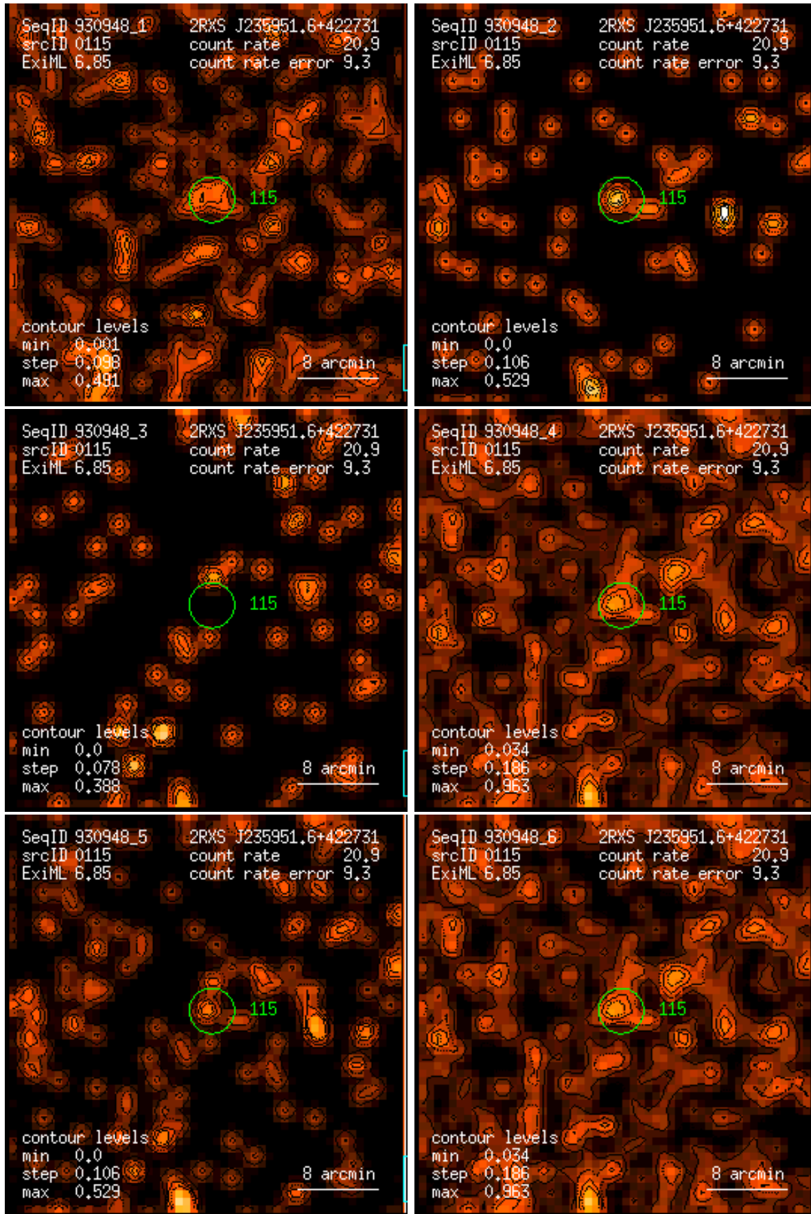
Figure 115: RASS 930948: detection 0115: band rate images, Gaussian filter: (1) PSPC channels 11 – 41, (2) 52 – 90, (3) 91 – 201, (4) 11 – 235, (5) 52 – 201, (6) 11 – 201. Broad band rates in counts/ks. Band rate contour levels in counts/ks/arcmin 2 .
