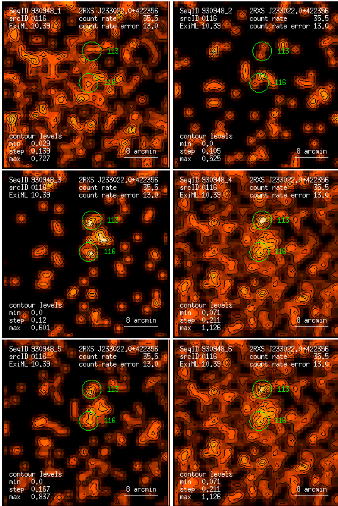
Figure 116: RASS 930948: detection 0116: band rate images, Gaussian filter: (1) PSPC channels 11 – 41, (2) 52 – 90, (3) 91 – 201, (4) 11 – 235, (5) 52 – 201, (6) 11 – 201. Broad band rates in counts/ks. Band rate contour levels in counts/ks/arcmin 2 .
