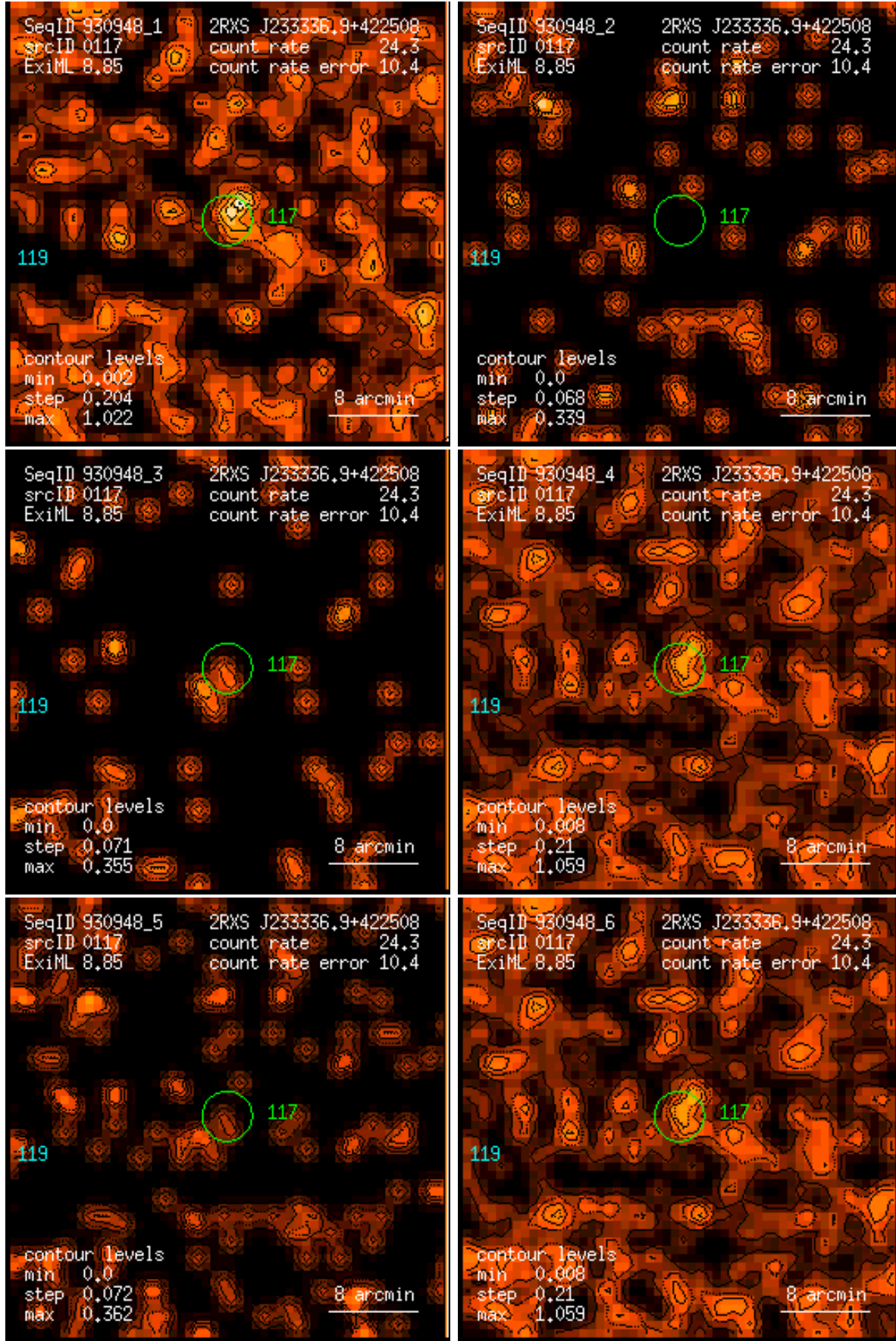
Figure 117: RASS 930948: detection 0117: band rate images, Gaussian filter: (1) PSPC channels 11 – 41, (2) 52 – 90, (3) 91 – 201, (4) 11 – 235, (5) 52 – 201, (6) 11 – 201. Broad band rates in counts/ks. Band rate contour levels in counts/ks/arcmin 2 .
