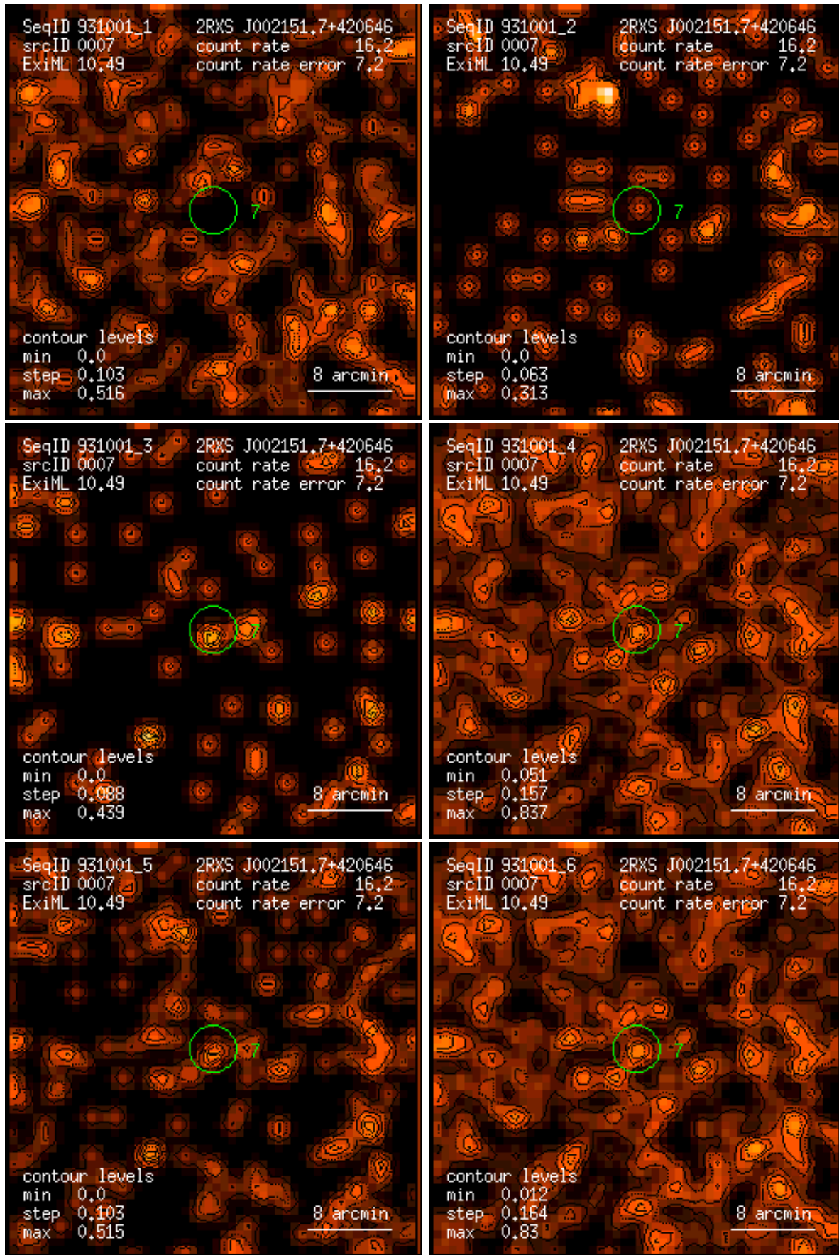
Figure 7: RASS 931001: detection 0007: band rate images, Gaussian filter: (1) PSPC channels 11 – 41, (2) 52 – 90, (3) 91 – 201, (4) 11 – 235, (5) 52 – 201, (6) 11 – 201. Broad band rates in counts/ks. Band rate contour levels in counts/ks/arcmin 2 .
