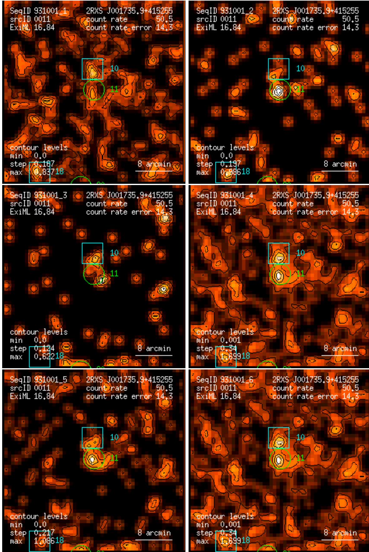
Figure 11: RASS 931001: detection 0011: band rate images, Gaussian filter: (1) PSPC channels 11 – 41, (2) 52 – 90, (3) 91 – 201, (4) 11 – 235, (5) 52 – 201, (6) 11 – 201. Broad band rates in counts/ks. Band rate contour levels in counts/ks/arcmin 2 .
