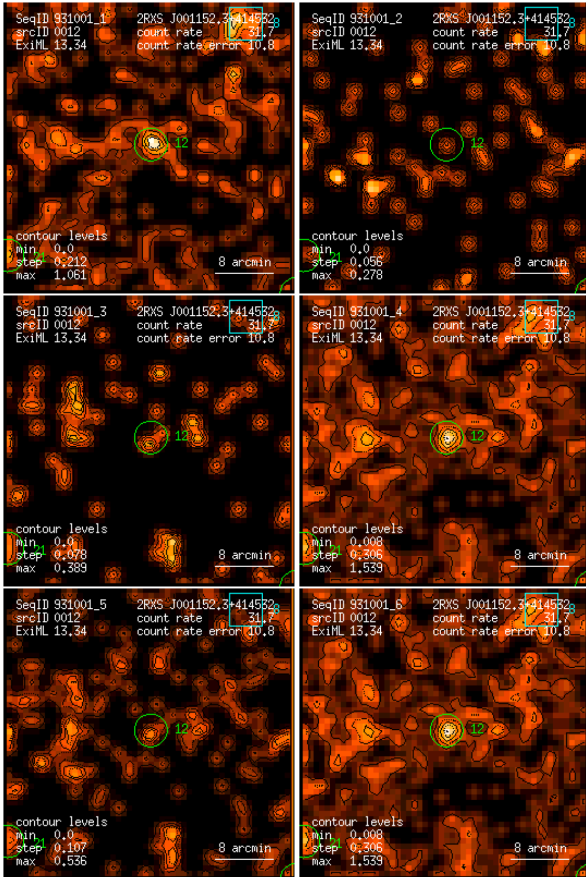
Figure 12: RASS 931001: detection 0012: band rate images, Gaussian filter: (1) PSPC channels 11 – 41, (2) 52 – 90, (3) 91 – 201, (4) 11 – 235, (5) 52 – 201, (6) 11 – 201. Broad band rates in counts/ks. Band rate contour levels in counts/ks/arcmin 2 .
