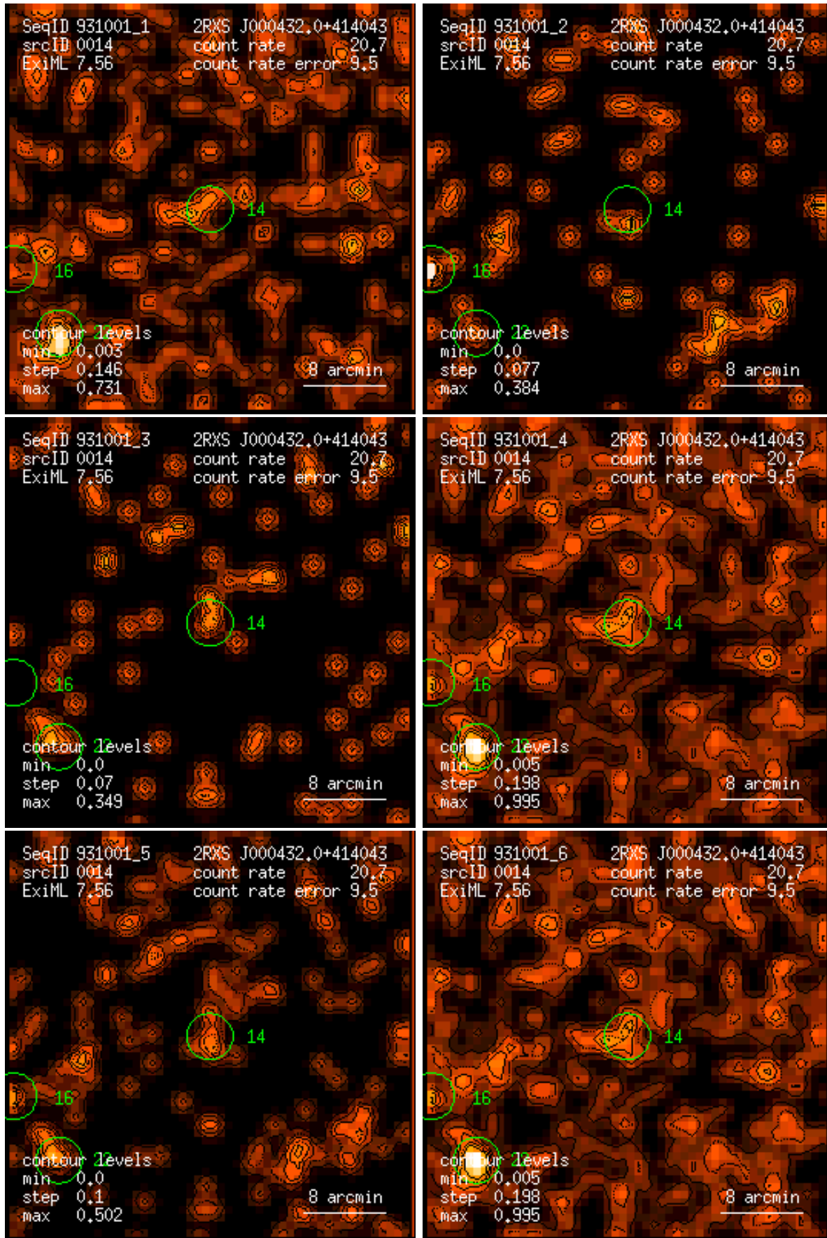
Figure 14: RASS 931001: detection 0014: band rate images, Gaussian filter: (1) PSPC channels 11 – 41, (2) 52 – 90, (3) 91 – 201, (4) 11 – 235, (5) 52 – 201, (6) 11 – 201. Broad band rates in counts/ks. Band rate contour levels in counts/ks/arcmin 2 .
