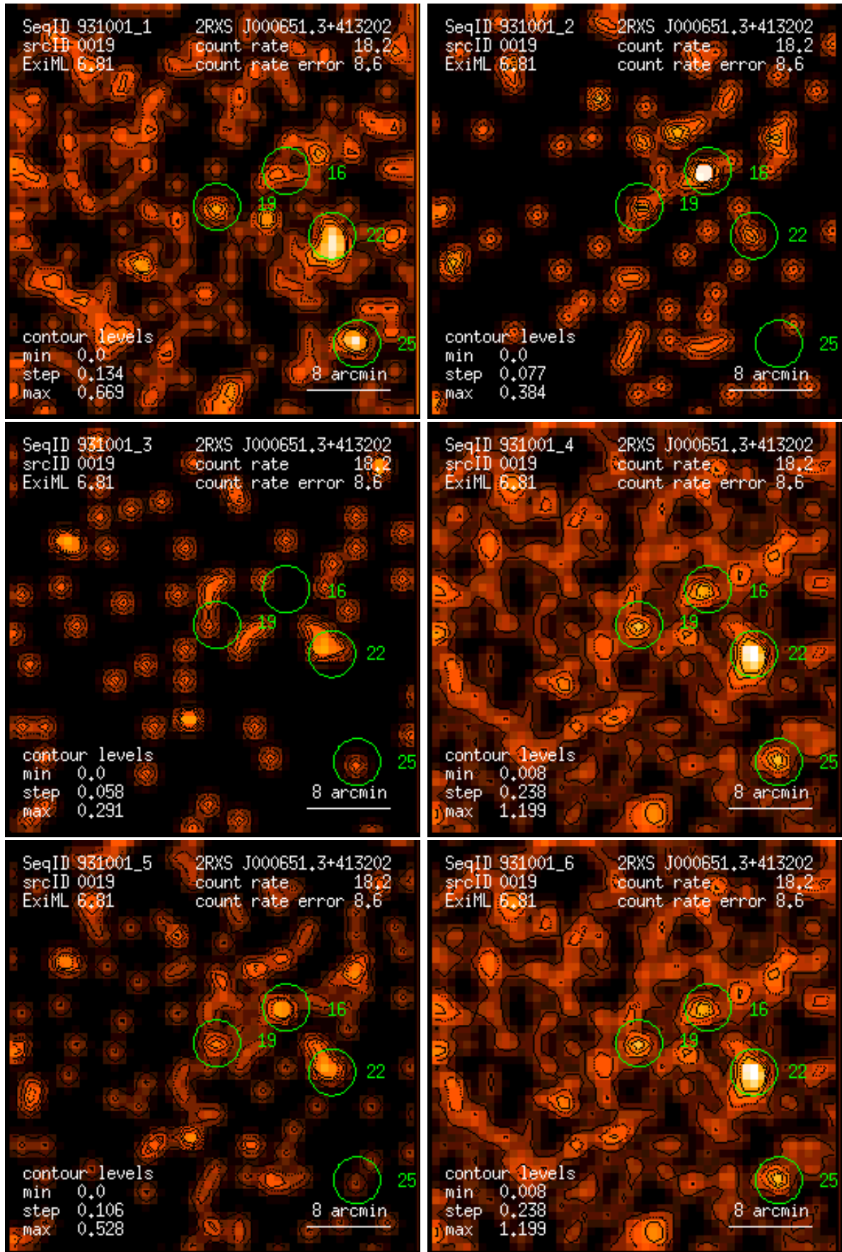
Figure 19: RASS 931001: detection 0019: band rate images, Gaussian filter: (1) PSPC channels 11 – 41, (2) 52 – 90, (3) 91 – 201, (4) 11 – 235, (5) 52 – 201, (6) 11 – 201. Broad band rates in counts/ks. Band rate contour levels in counts/ks/arcmin 2 .
