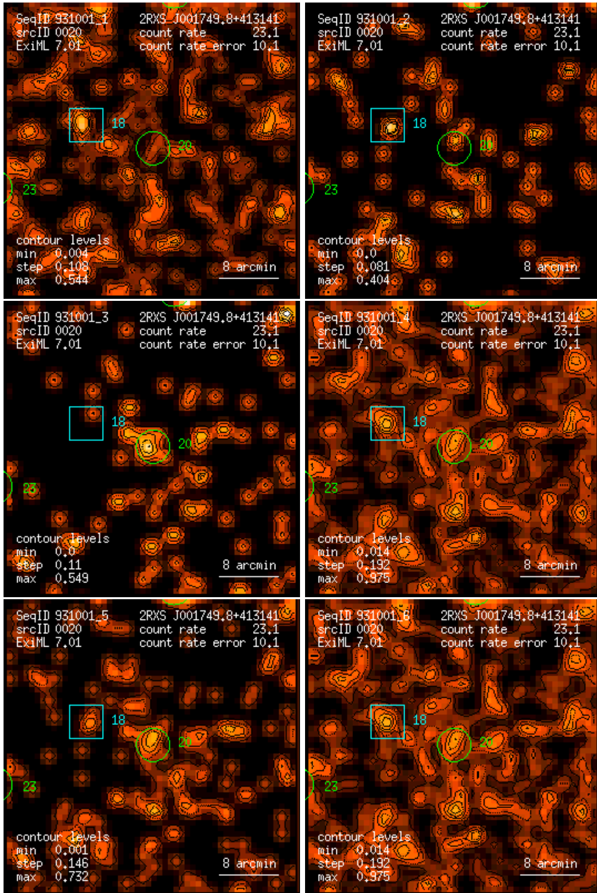
Figure 20: RASS 931001: detection 0020: band rate images, Gaussian filter: (1) PSPC channels 11 – 41, (2) 52 – 90, (3) 91 – 201, (4) 11 – 235, (5) 52 – 201, (6) 11 – 201. Broad band rates in counts/ks. Band rate contour levels in counts/ks/arcmin 2 .
