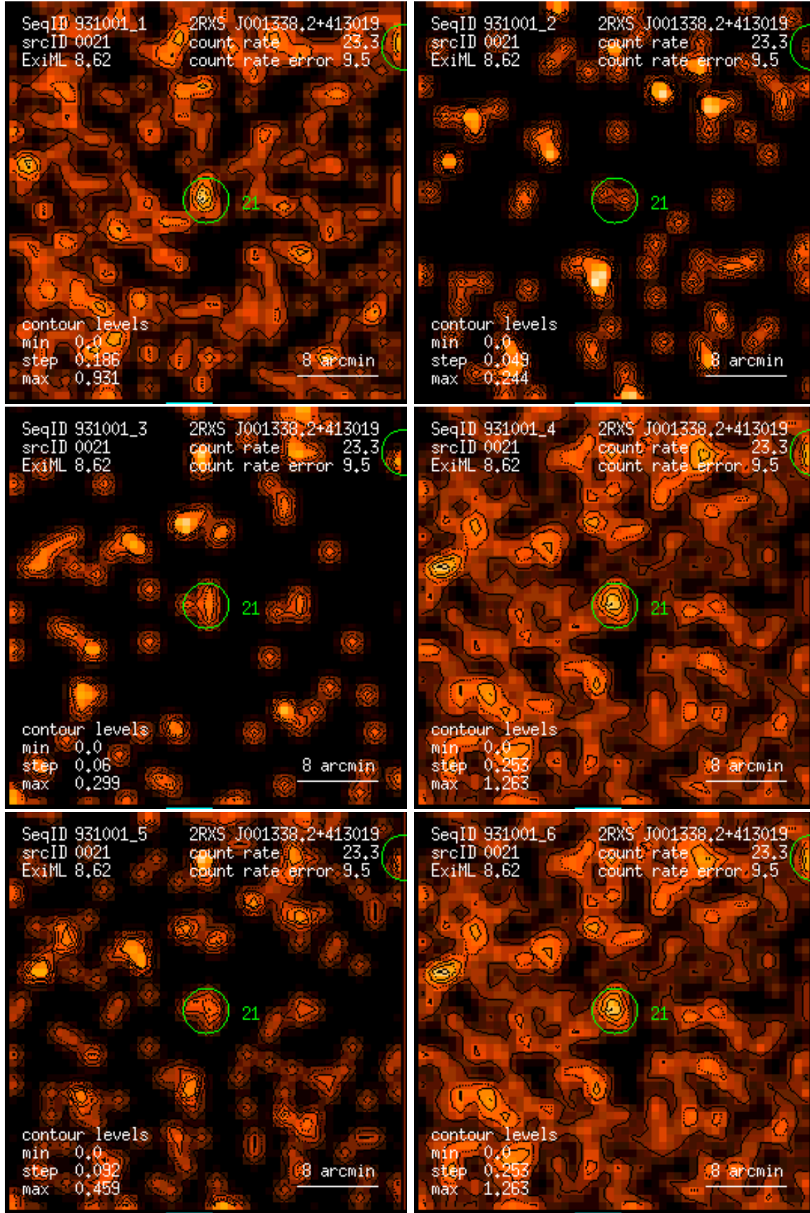
Figure 21: RASS 931001: detection 0021: band rate images, Gaussian filter: (1) PSPC channels 11 – 41, (2) 52 – 90, (3) 91 – 201, (4) 11 – 235, (5) 52 – 201, (6) 11 – 201. Broad band rates in counts/ks. Band rate contour levels in counts/ks/arcmin 2 .
