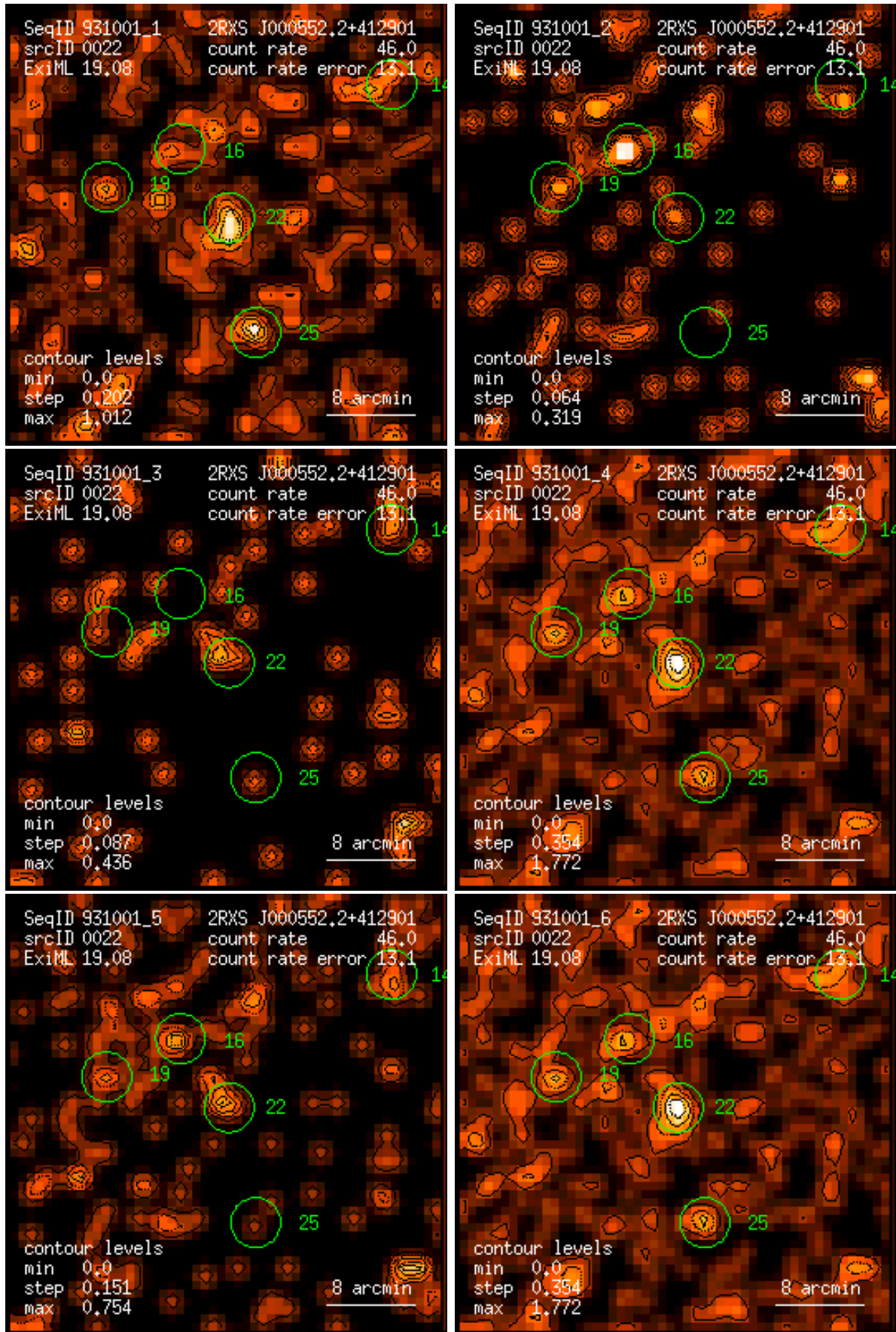
Figure 22: RASS 931001: detection 0022: band rate images, Gaussian filter: (1) PSPC channels 11 – 41, (2) 52 – 90, (3) 91 – 201, (4) 11 – 235, (5) 52 – 201, (6) 11 – 201. Broad band rates in counts/ks. Band rate contour levels in counts/ks/arcmin 2 .
