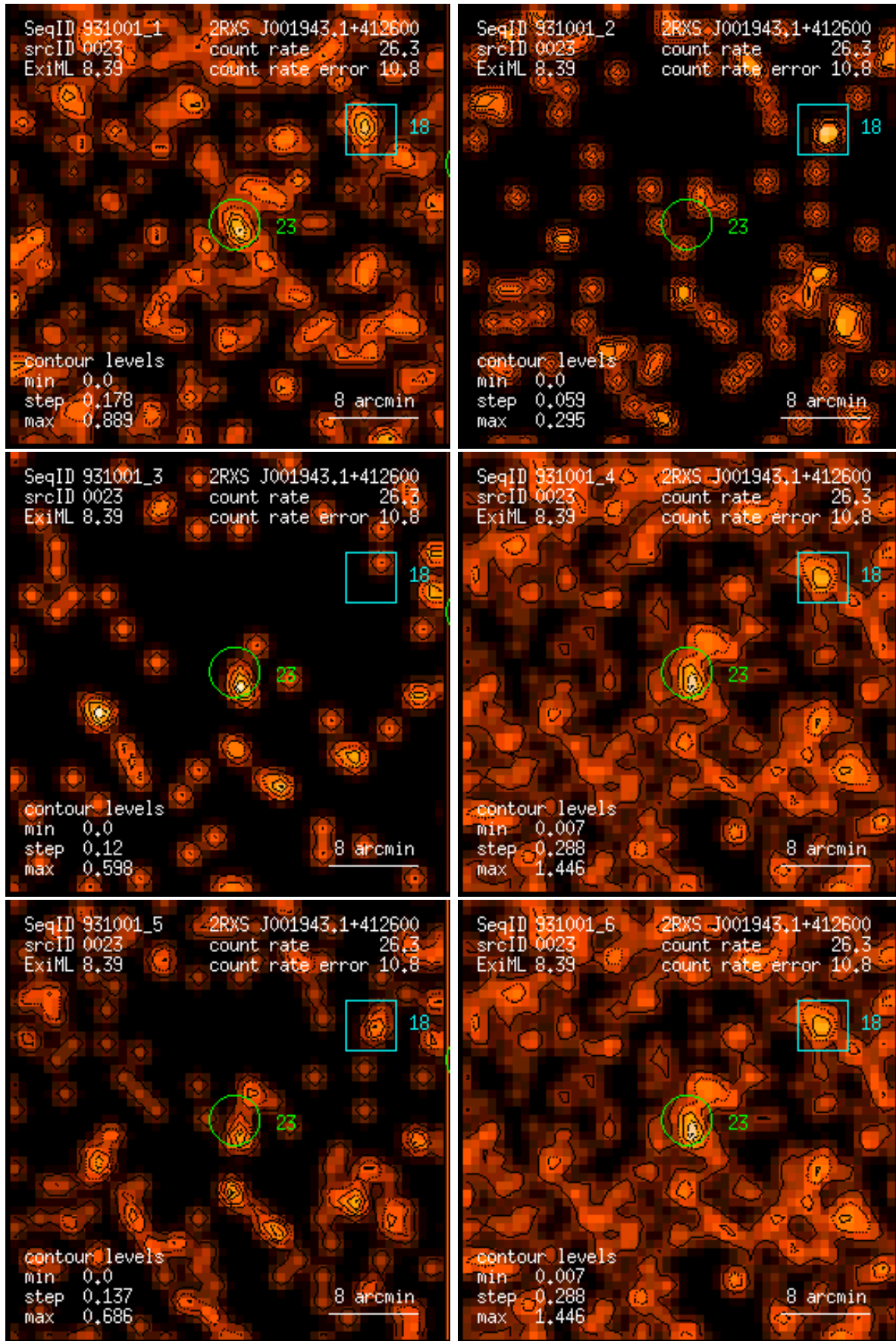
Figure 23: RASS 931001: detection 0023: band rate images, Gaussian filter: (1) PSPC channels 11 – 41, (2) 52 – 90, (3) 91 – 201, (4) 11 – 235, (5) 52 – 201, (6) 11 – 201. Broad band rates in counts/ks. Band rate contour levels in counts/ks/arcmin 2 .
