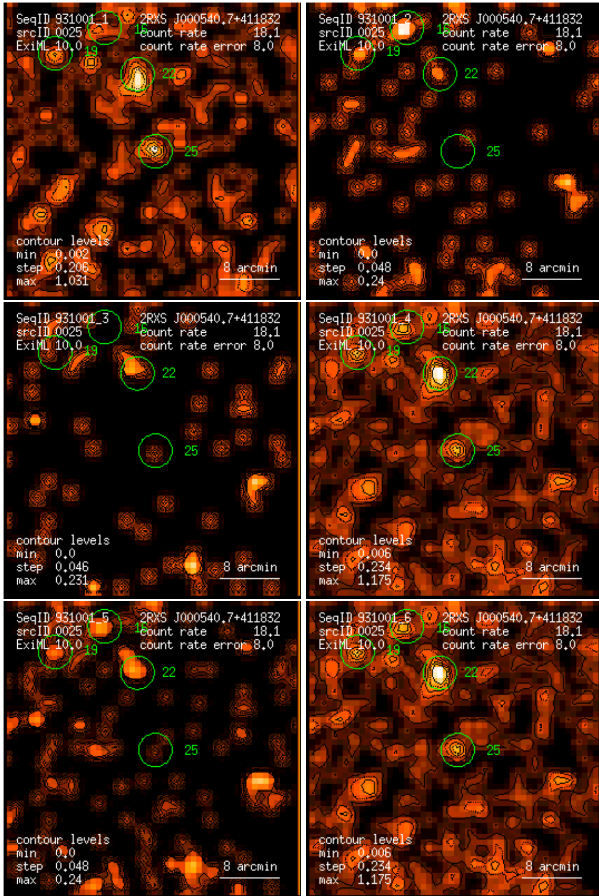
Figure 25: RASS 931001: detection 0025: band rate images, Gaussian filter: (1) PSPC channels 11 – 41, (2) 52 – 90, (3) 91 – 201, (4) 11 – 235, (5) 52 – 201, (6) 11 – 201. Broad band rates in counts/ks. Band rate contour levels in counts/ks/arcmin 2 .
