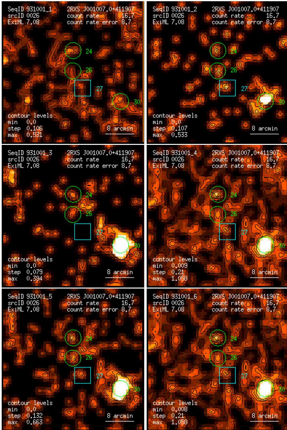
Figure 26: RASS 931001: detection 0026: band rate images, Gaussian filter: (1) PSPC channels 11 – 41, (2) 52 – 90, (3) 91 – 201, (4) 11 – 235, (5) 52 – 201, (6) 11 – 201. Broad band rates in counts/ks. Band rate contour levels in counts/ks/arcmin 2 .
