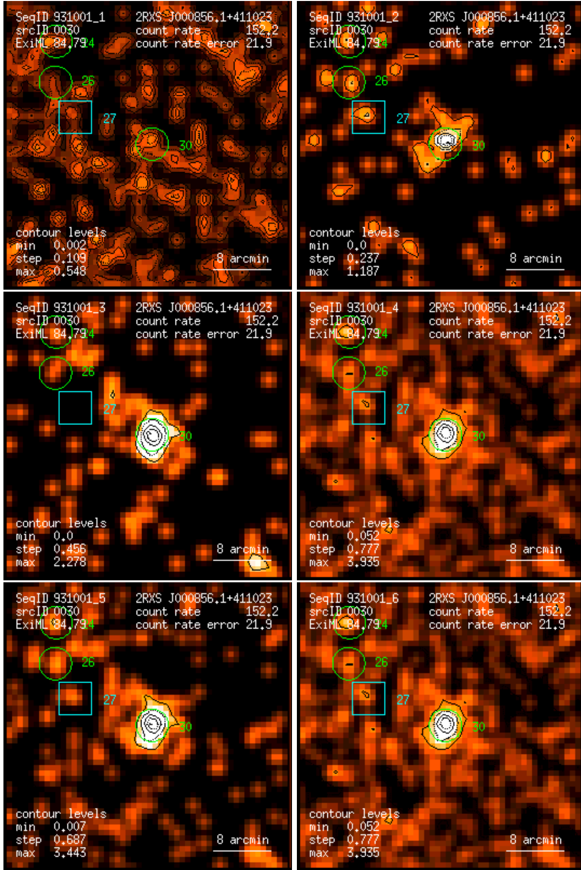
Figure 30: RASS 931001: detection 0030: band rate images, Gaussian filter: (1) PSPC channels 11 – 41, (2) 52 – 90, (3) 91 – 201, (4) 11 – 235, (5) 52 – 201, (6) 11 – 201. Broad band rates in counts/ks. Band rate contour levels in counts/ks/arcmin 2 .
