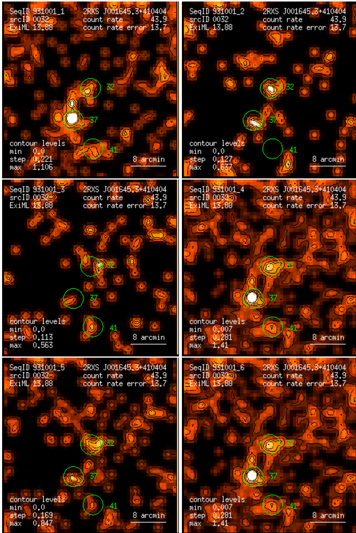
Figure 32: RASS 931001: detection 0032: band rate images, Gaussian filter: (1) PSPC channels 11 – 41, (2) 52 – 90, (3) 91 – 201, (4) 11 – 235, (5) 52 – 201, (6) 11 – 201. Broad band rates in counts/ks. Band rate contour levels in counts/ks/arcmin 2 .
