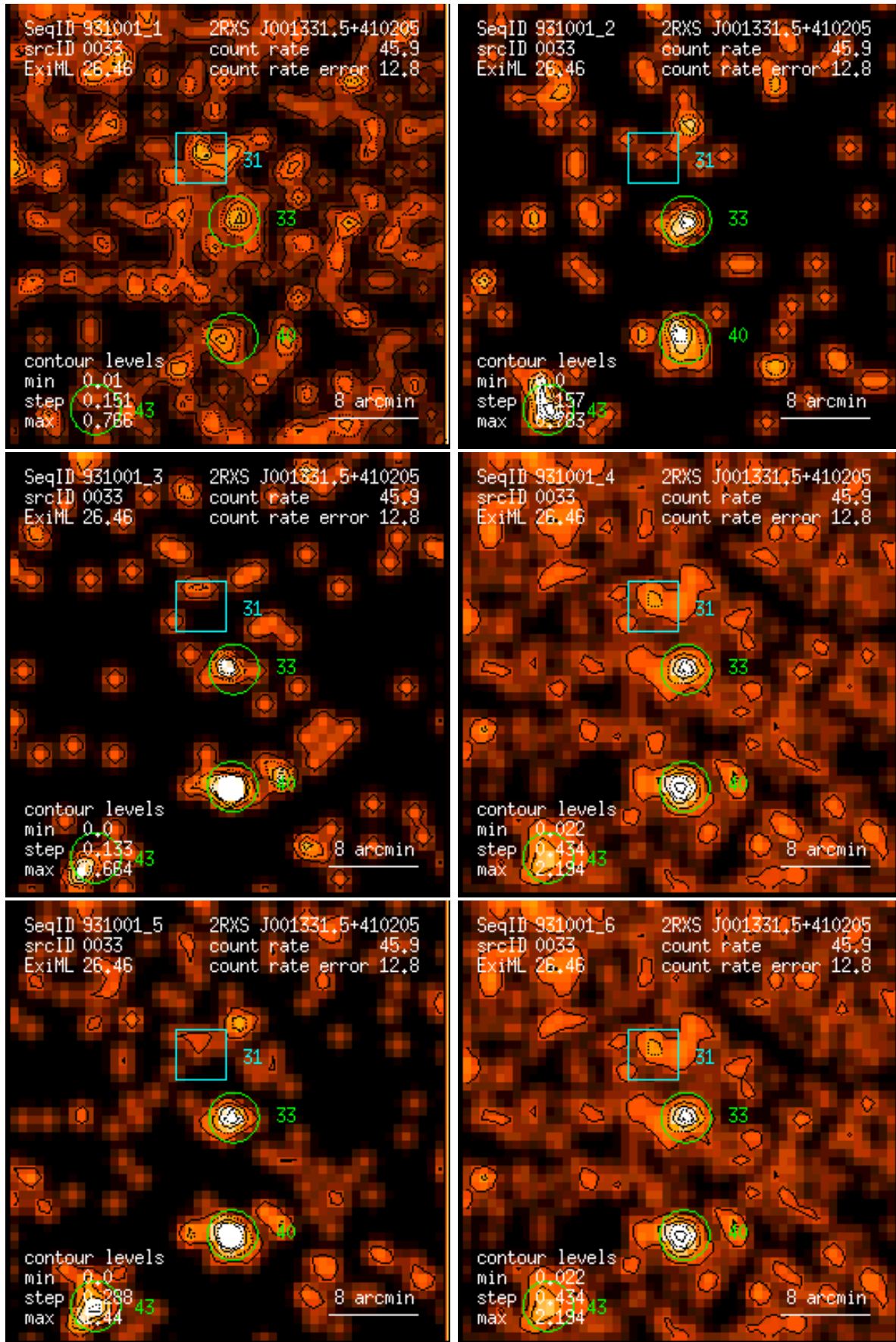
Figure 33: RASS 931001: detection 0033: band rate images, Gaussian filter: (1) PSPC channels 11 – 41, (2) 52 – 90, (3) 91 – 201, (4) 11 – 235, (5) 52 – 201, (6) 11 – 201. Broad band rates in counts/ks. Band rate contour levels in counts/ks/arcmin 2 .
