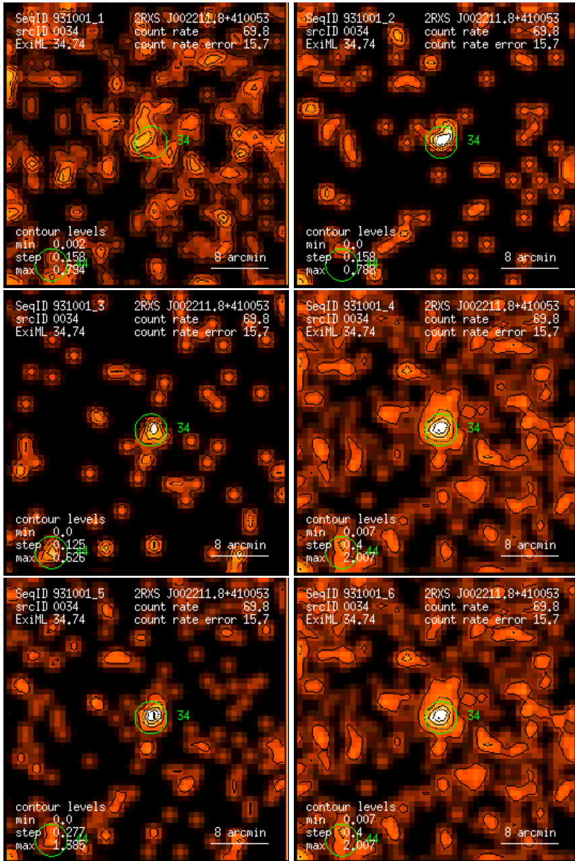
Figure 34: RASS 931001: detection 0034: band rate images, Gaussian filter: (1) PSPC channels 11 – 41, (2) 52 – 90, (3) 91 – 201, (4) 11 – 235, (5) 52 – 201, (6) 11 – 201. Broad band rates in counts/ks. Band rate contour levels in counts/ks/arcmin 2 .
