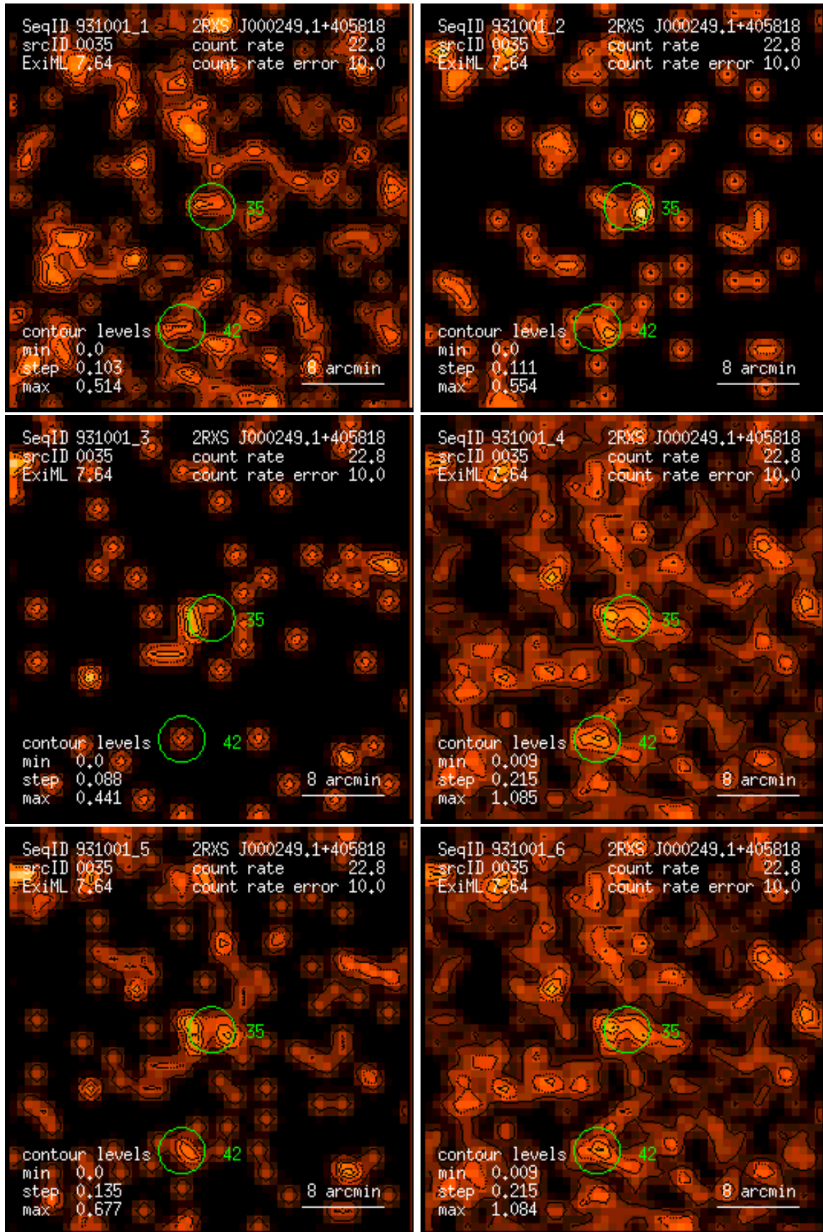
Figure 35: RASS 931001: detection 0035: band rate images, Gaussian filter: (1) PSPC channels 11 – 41, (2) 52 – 90, (3) 91 – 201, (4) 11 – 235, (5) 52 – 201, (6) 11 – 201. Broad band rates in counts/ks. Band rate contour levels in counts/ks/arcmin 2 .
