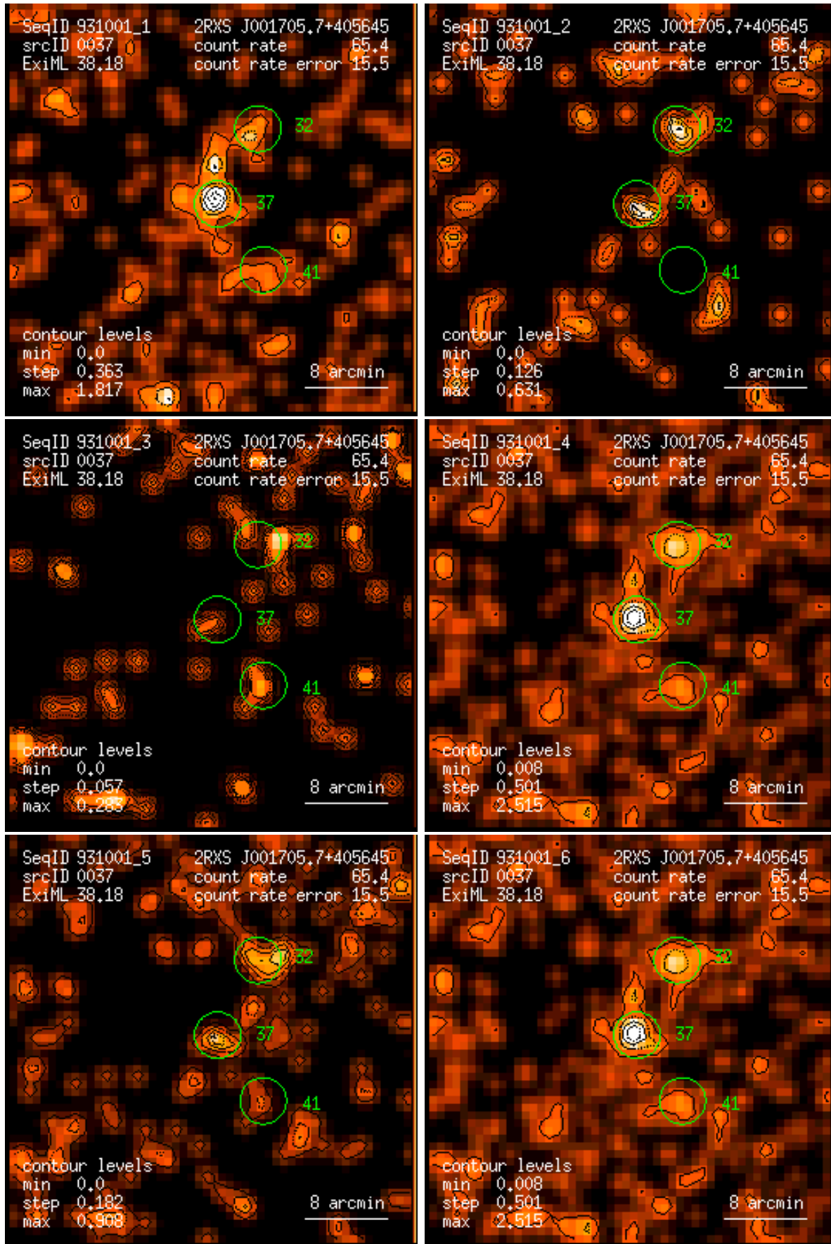
Figure 37: RASS 931001: detection 0037: band rate images, Gaussian filter: (1) PSPC channels 11 – 41, (2) 52 – 90, (3) 91 – 201, (4) 11 – 235, (5) 52 – 201, (6) 11 – 201. Broad band rates in counts/ks. Band rate contour levels in counts/ks/arcmin 2 .
