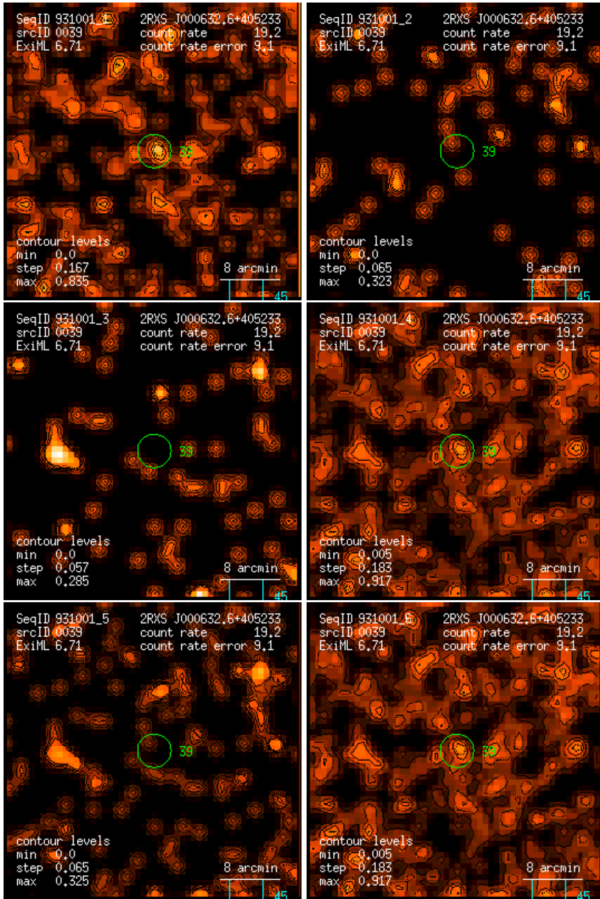
Figure 39: RASS 931001: detection 0039: band rate images, Gaussian filter: (1) PSPC channels 11 – 41, (2) 52 – 90, (3) 91 – 201, (4) 11 – 235, (5) 52 – 201, (6) 11 – 201. Broad band rates in counts/ks. Band rate contour levels in counts/ks/arcmin 2 .
