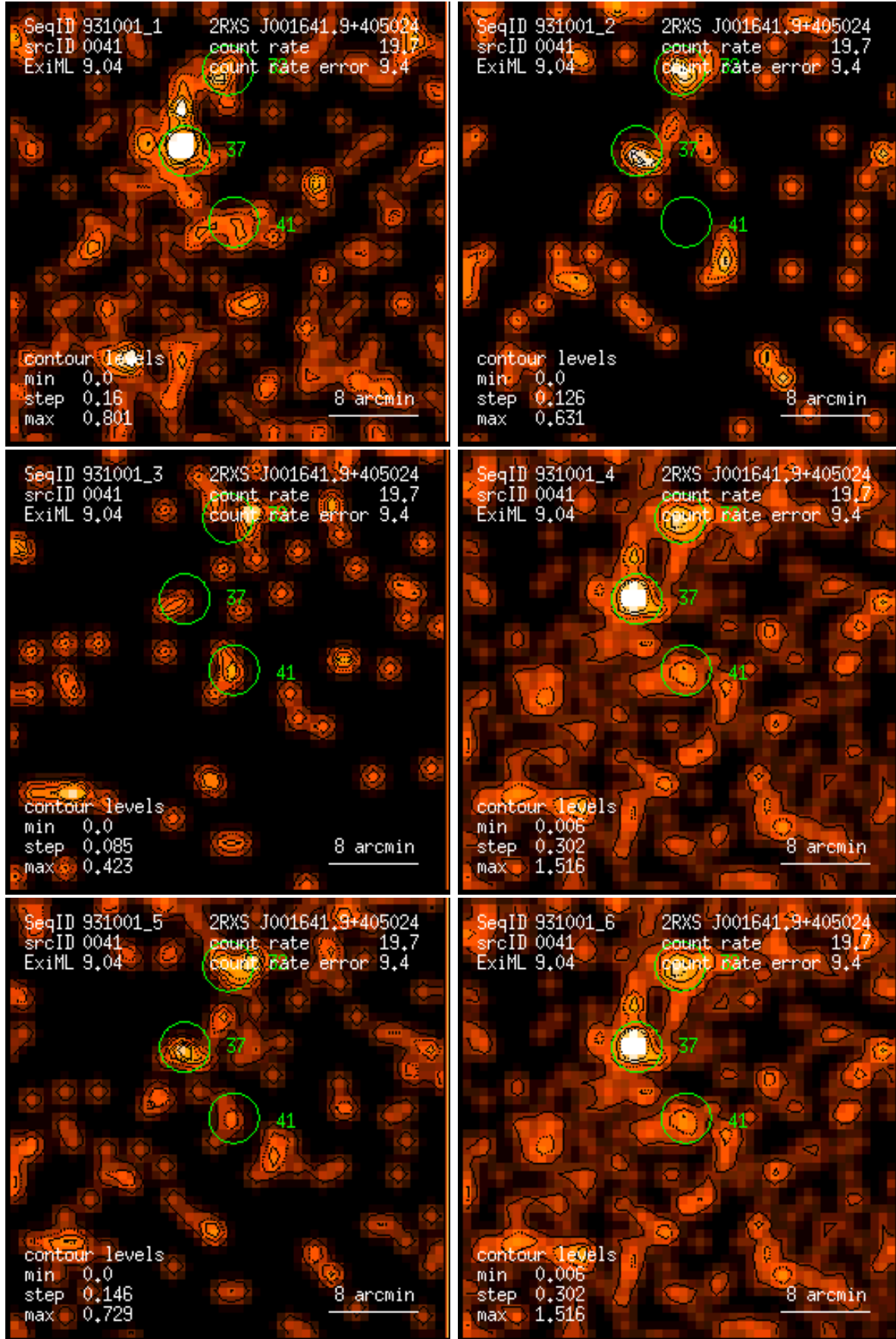
Figure 41: RASS 931001: detection 0041: band rate images, Gaussian filter: (1) PSPC channels 11 – 41, (2) 52 – 90, (3) 91 – 201, (4) 11 – 235, (5) 52 – 201, (6) 11 – 201. Broad band rates in counts/ks. Band rate contour levels in counts/ks/arcmin 2 .
