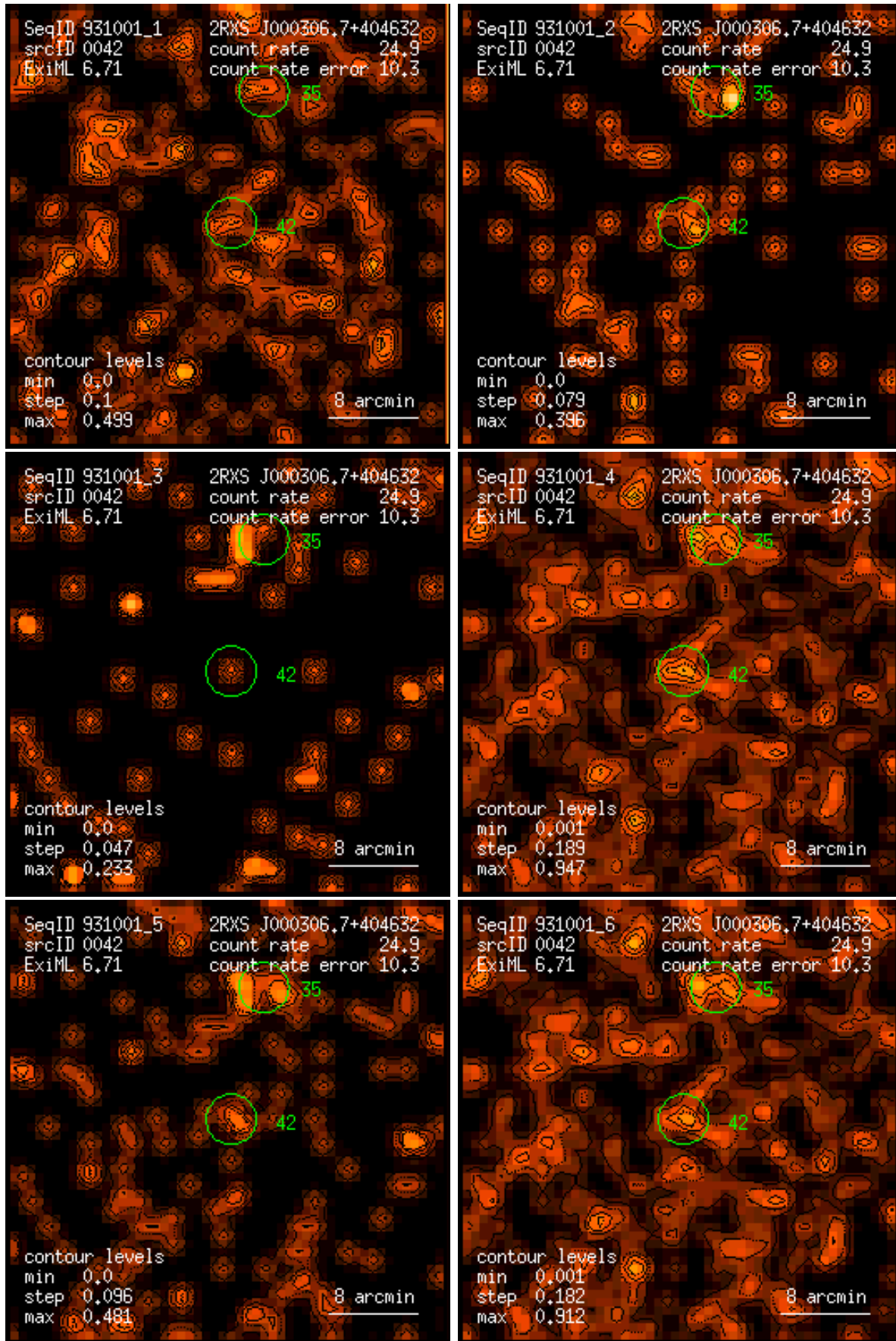
Figure 42: RASS 931001: detection 0042: band rate images, Gaussian filter: (1) PSPC channels 11 – 41, (2) 52 – 90, (3) 91 – 201, (4) 11 – 235, (5) 52 – 201, (6) 11 – 201. Broad band rates in counts/ks. Band rate contour levels in counts/ks/arcmin 2 .
