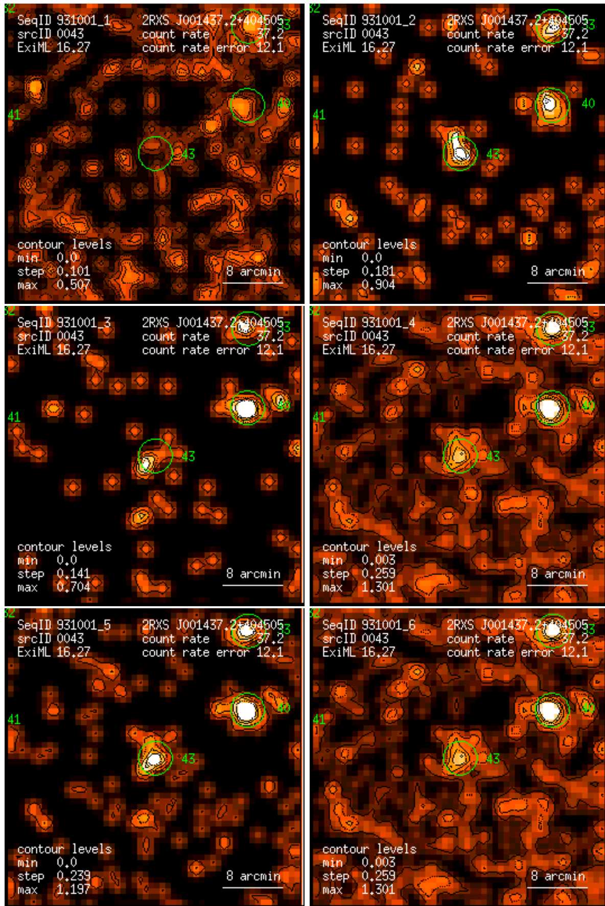
Figure 43: RASS 931001: detection 0043: band rate images, Gaussian filter: (1) PSPC channels 11 – 41, (2) 52 – 90, (3) 91 – 201, (4) 11 – 235, (5) 52 – 201, (6) 11 – 201. Broad band rates in counts/ks. Band rate contour levels in counts/ks/arcmin 2 .
