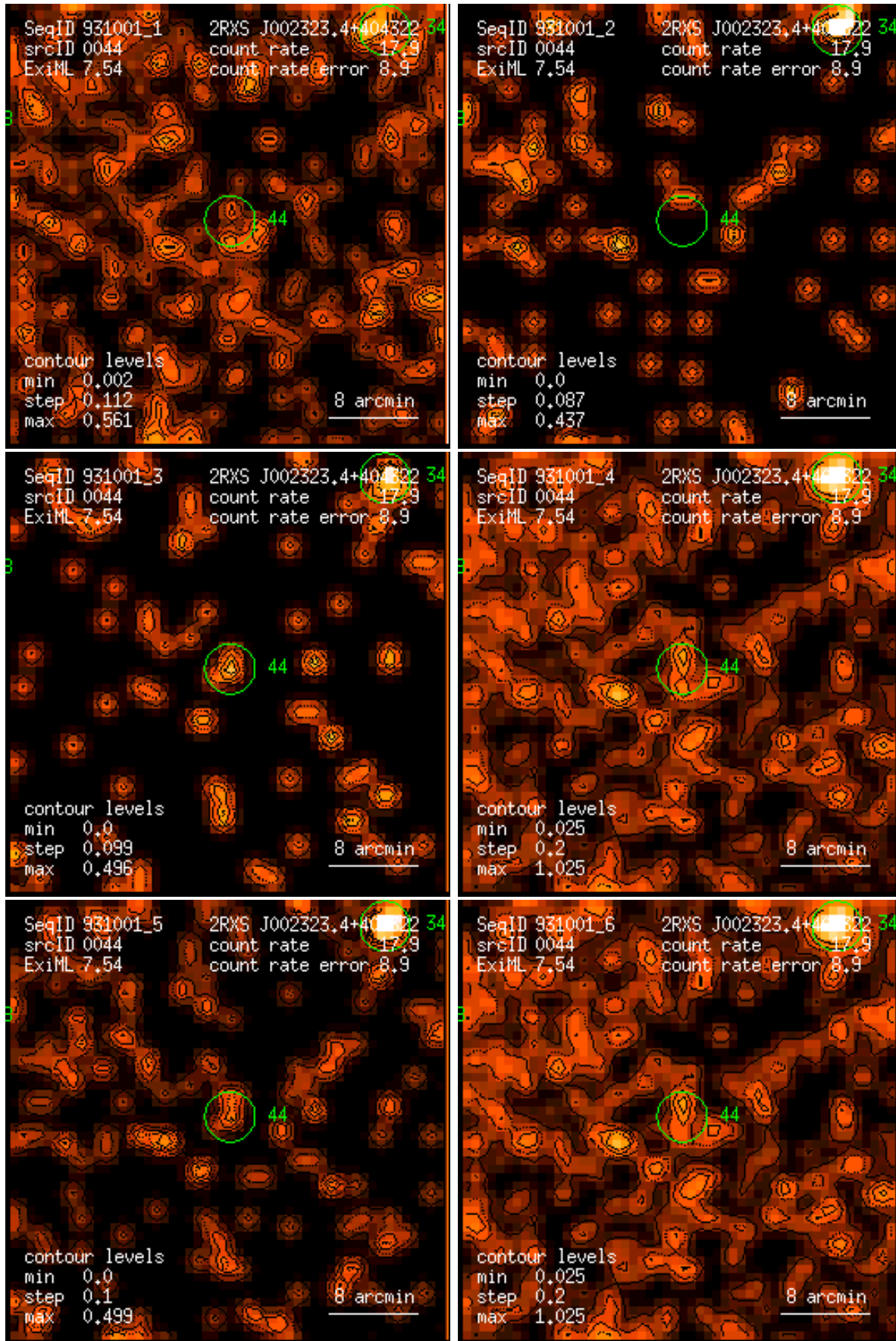
Figure 44: RASS 931001: detection 0044: band rate images, Gaussian filter: (1) PSPC channels 11 – 41, (2) 52 – 90, (3) 91 – 201, (4) 11 – 235, (5) 52 – 201, (6) 11 – 201. Broad band rates in counts/ks. Band rate contour levels in counts/ks/arcmin 2 .
