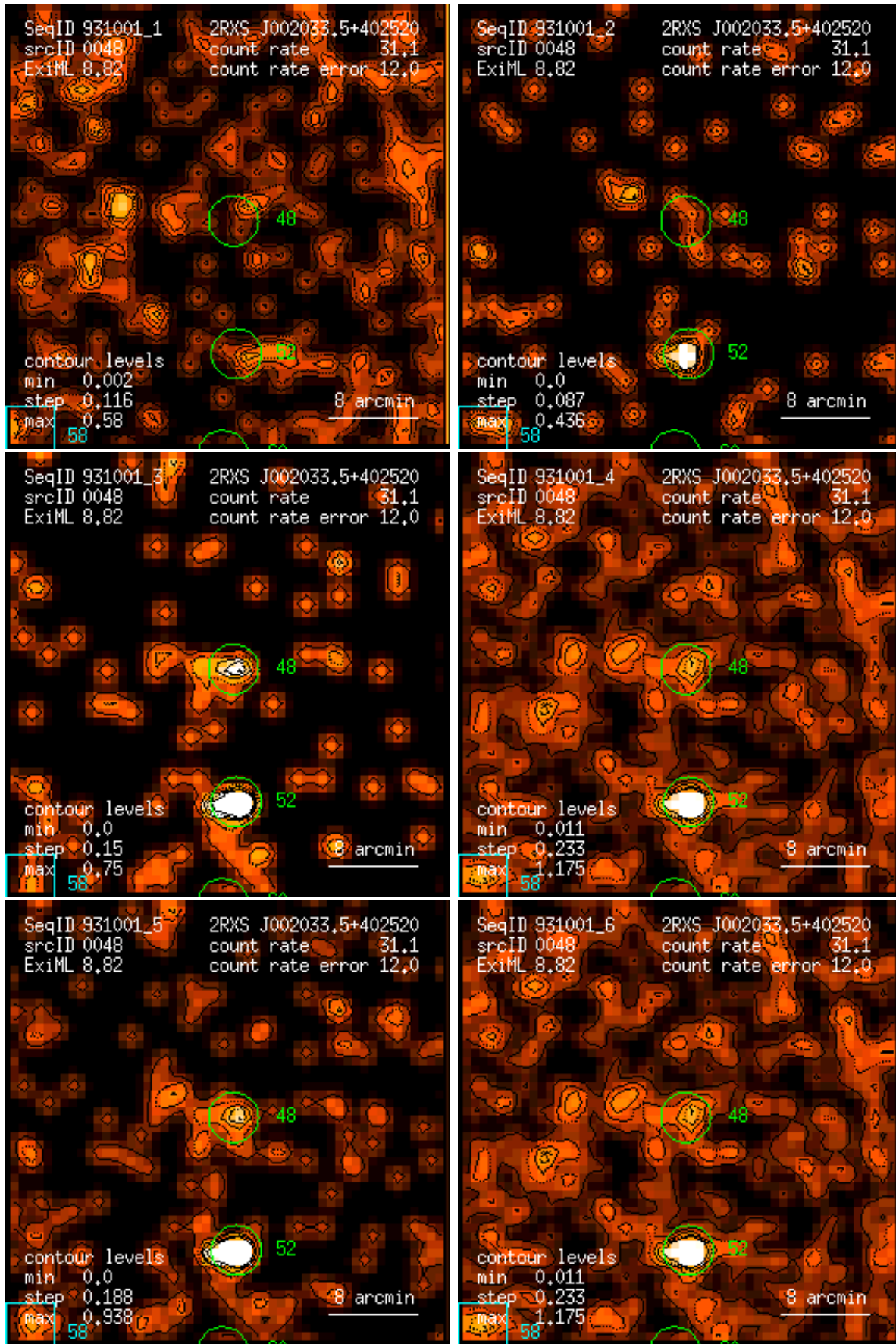
Figure 48: RASS 931001: detection 0048: band rate images, Gaussian filter: (1) PSPC channels 11 – 41, (2) 52 – 90, (3) 91 – 201, (4) 11 – 235, (5) 52 – 201, (6) 11 – 201. Broad band rates in counts/ks. Band rate contour levels in counts/ks/arcmin 2 .
