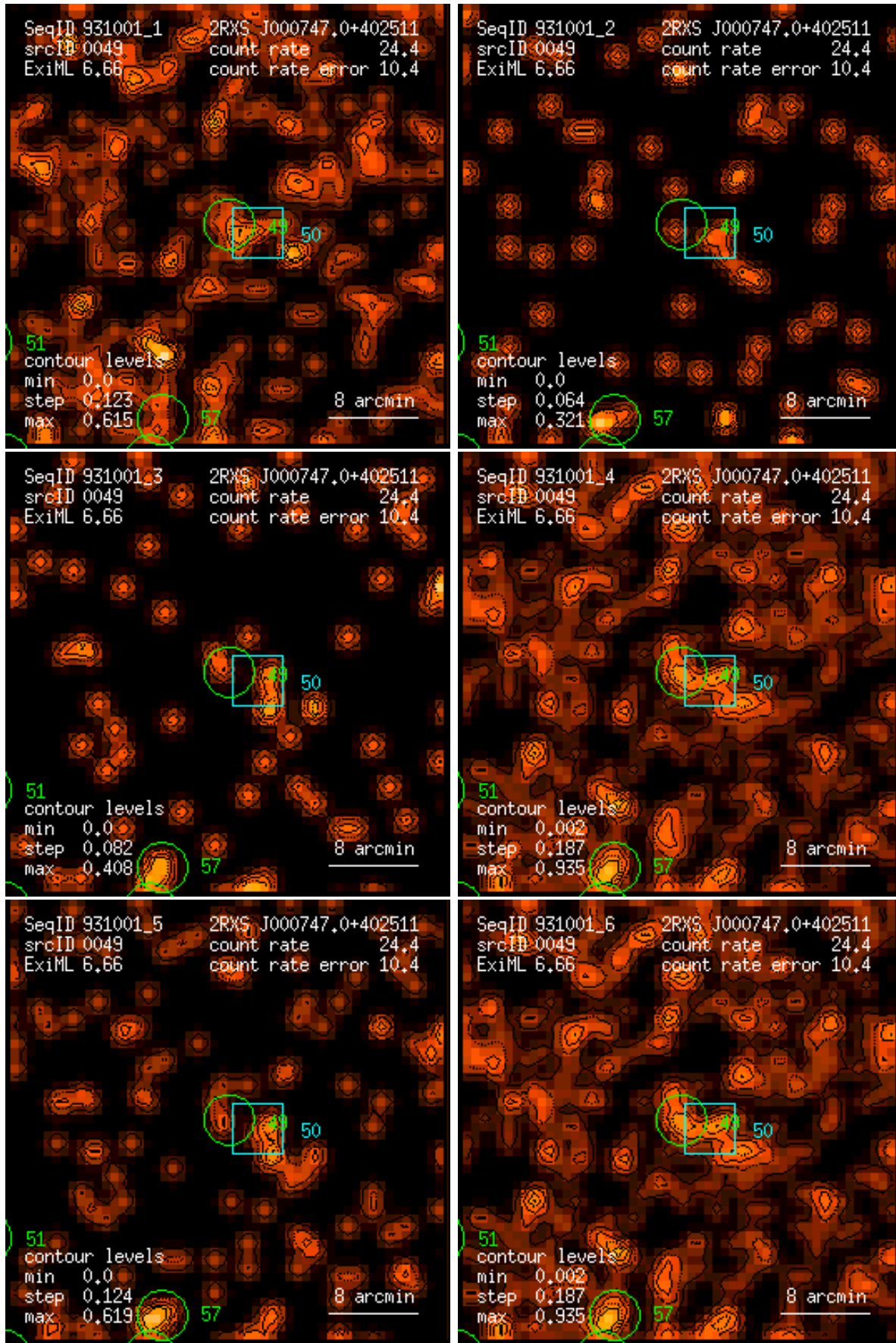
Figure 49: RASS 931001: detection 0049: band rate images, Gaussian filter: (1) PSPC channels 11 – 41, (2) 52 – 90, (3) 91 – 201, (4) 11 – 235, (5) 52 – 201, (6) 11 – 201. Broad band rates in counts/ks. Band rate contour levels in counts/ks/arcmin 2 .
