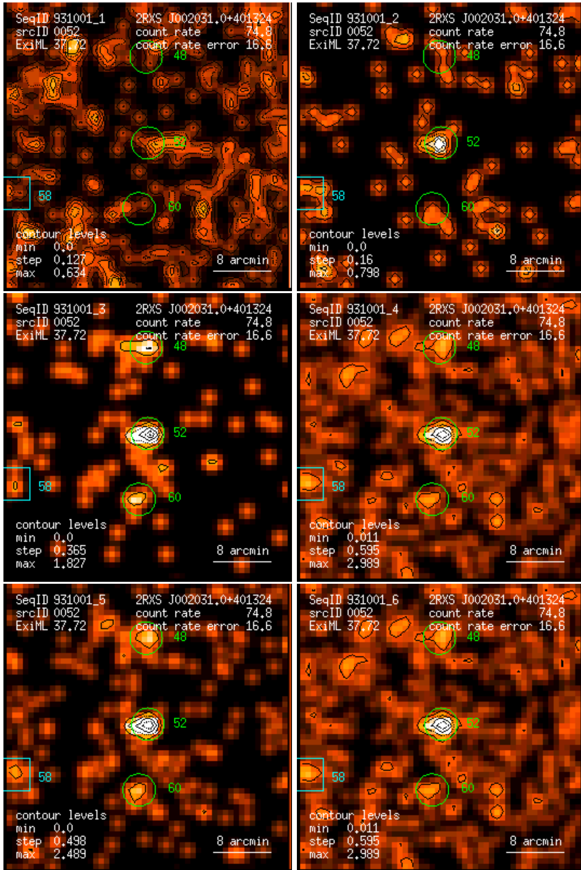
Figure 52: RASS 931001: detection 0052: band rate images, Gaussian filter: (1) PSPC channels 11 – 41, (2) 52 – 90, (3) 91 – 201, (4) 11 – 235, (5) 52 – 201, (6) 11 – 201. Broad band rates in counts/ks. Band rate contour levels in counts/ks/arcmin 2 .
