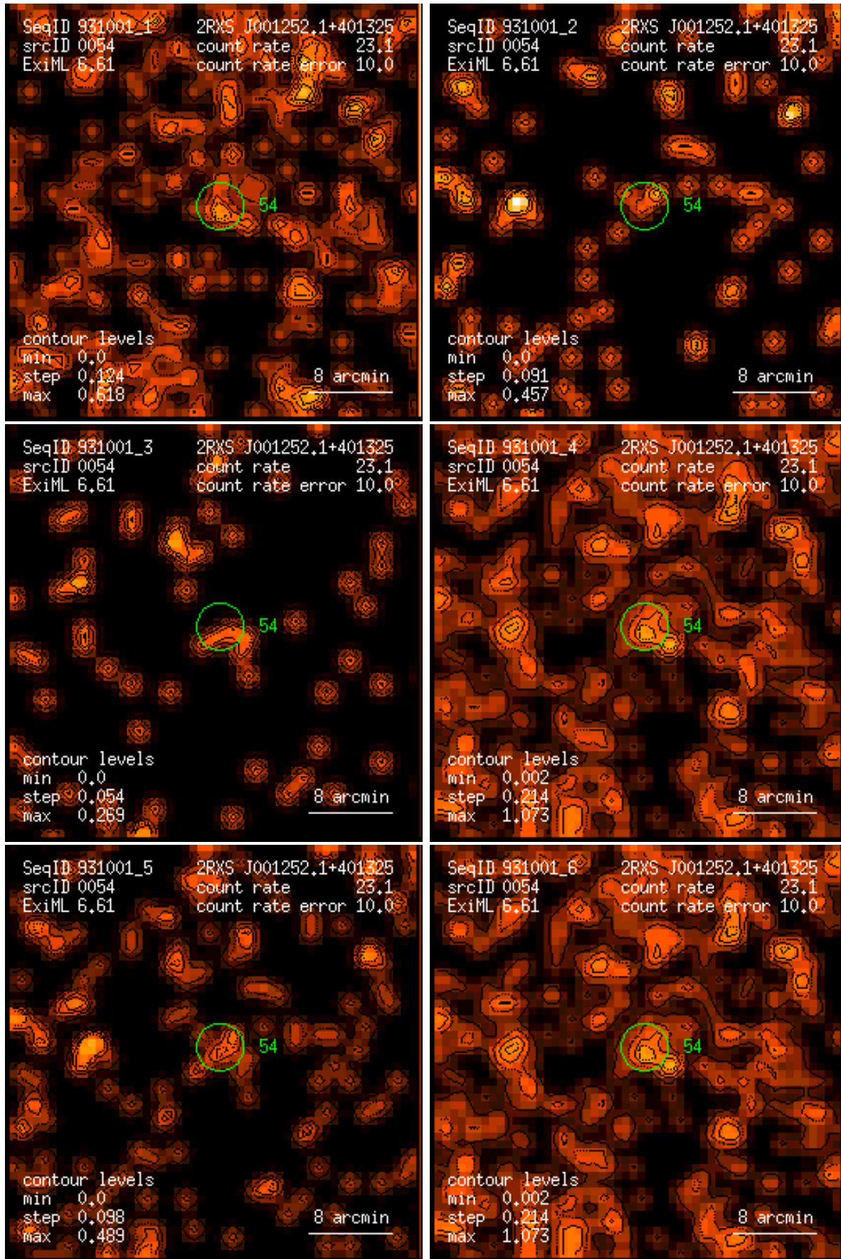
Figure 54: RASS 931001: detection 0054: band rate images, Gaussian filter: (1) PSPC channels 11 – 41, (2) 52 – 90, (3) 91 – 201, (4) 11 – 235, (5) 52 – 201, (6) 11 – 201. Broad band rates in counts/ks. Band rate contour levels in counts/ks/arcmin 2 .
