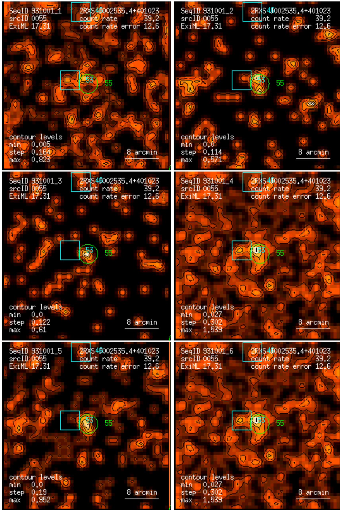
Figure 55: RASS 931001: detection 0055: band rate images, Gaussian filter: (1) PSPC channels 11 – 41, (2) 52 – 90, (3) 91 – 201, (4) 11 – 235, (5) 52 – 201, (6) 11 – 201. Broad band rates in counts/ks. Band rate contour levels in counts/ks/arcmin 2 .
