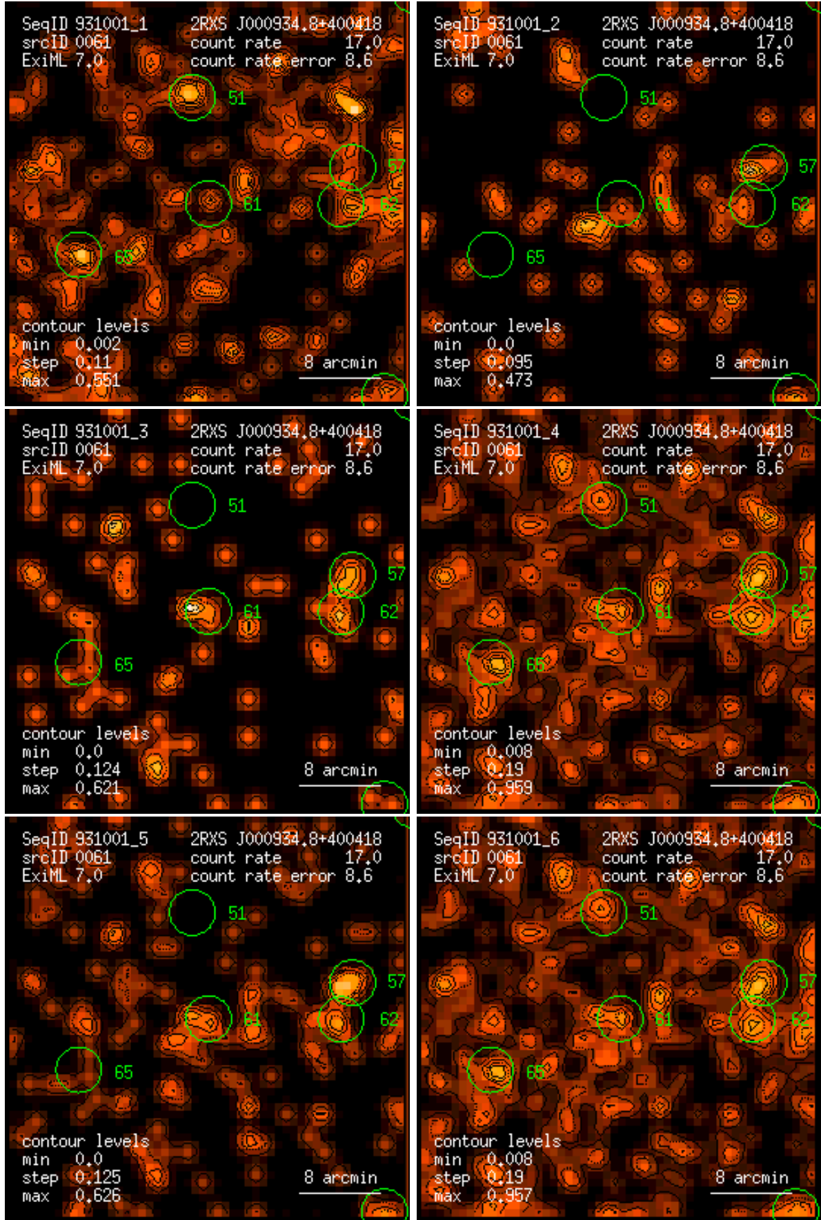
Figure 61: RASS 931001: detection 0061: band rate images, Gaussian filter: (1) PSPC channels 11 – 41, (2) 52 – 90, (3) 91 – 201, (4) 11 – 235, (5) 52 – 201, (6) 11 – 201. Broad band rates in counts/ks. Band rate contour levels in counts/ks/arcmin 2 .
