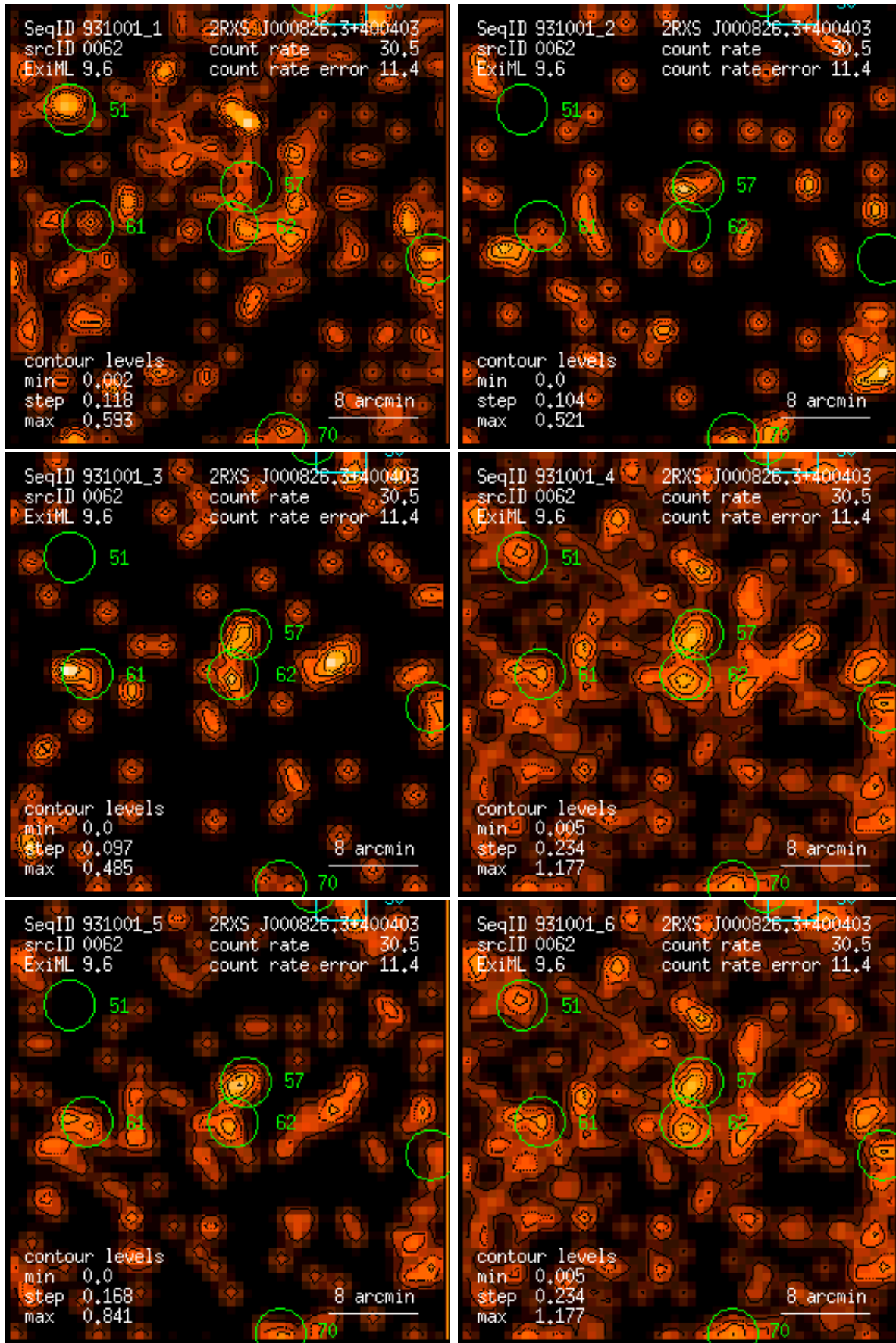
Figure 62: RASS 931001: detection 0062: band rate images, Gaussian filter: (1) PSPC channels 11 – 41, (2) 52 – 90, (3) 91 – 201, (4) 11 – 235, (5) 52 – 201, (6) 11 – 201. Broad band rates in counts/ks. Band rate contour levels in counts/ks/arcmin 2 .
