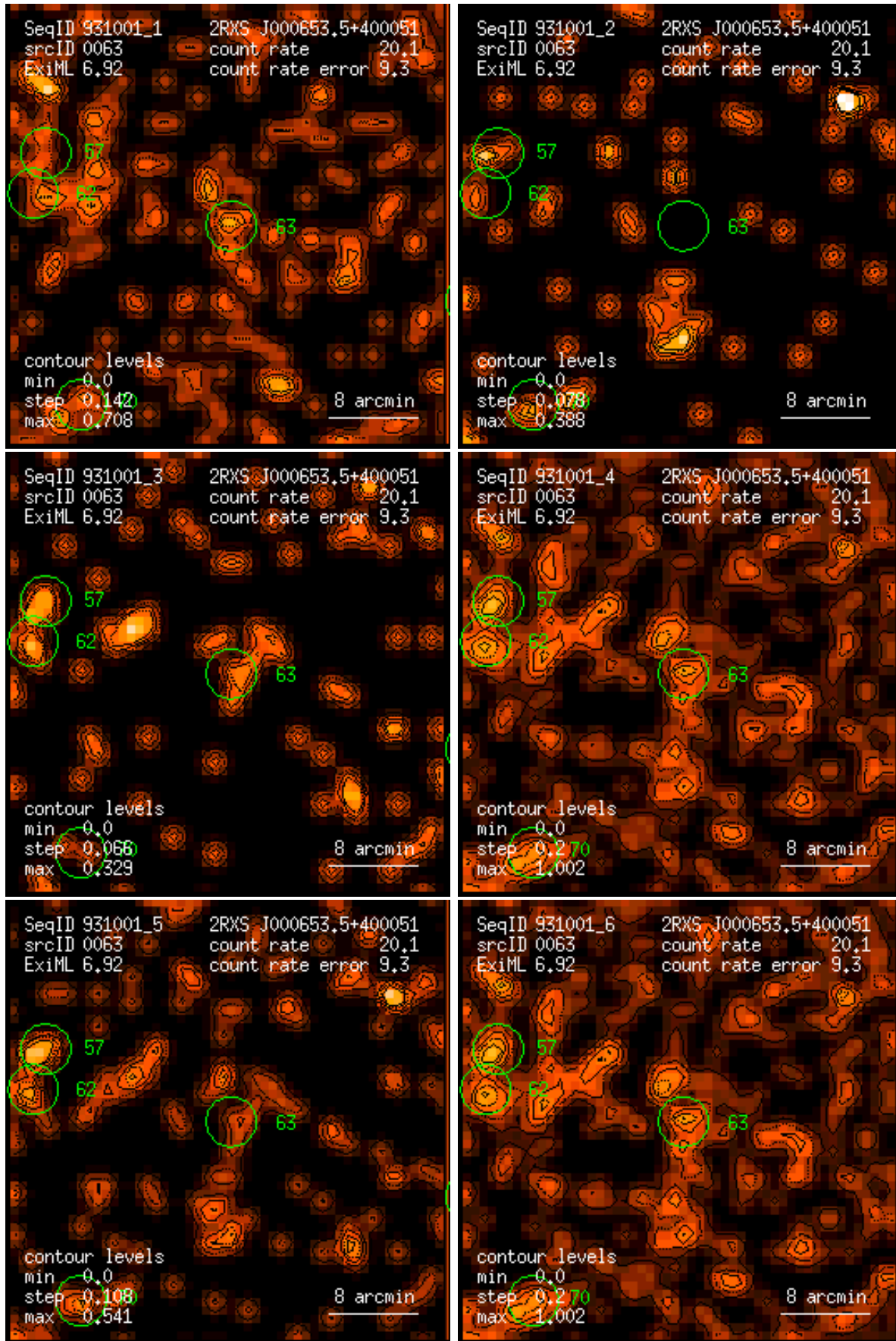
Figure 63: RASS 931001: detection 0063: band rate images, Gaussian filter: (1) PSPC channels 11 – 41, (2) 52 – 90, (3) 91 – 201, (4) 11 – 235, (5) 52 – 201, (6) 11 – 201. Broad band rates in counts/ks. Band rate contour levels in counts/ks/arcmin 2 .
