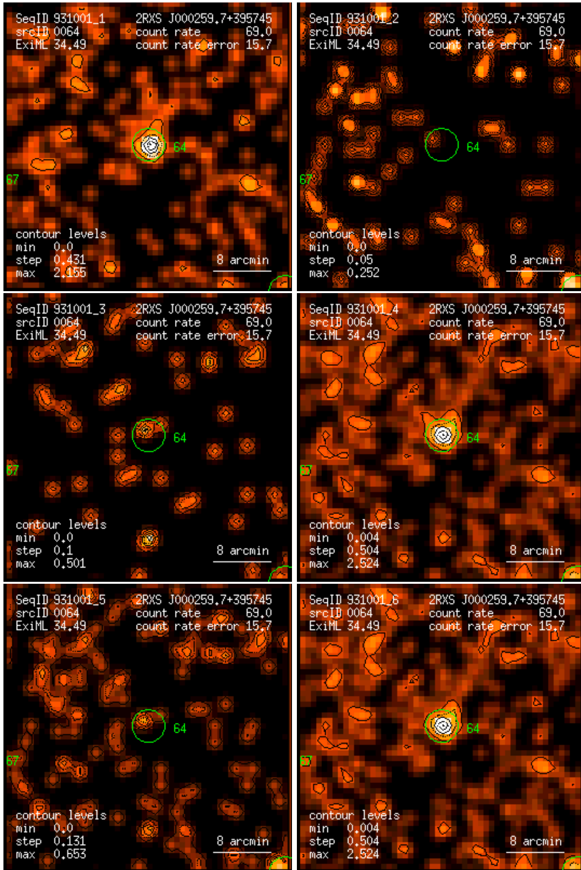
Figure 64: RASS 931001: detection 0064: band rate images, Gaussian filter: (1) PSPC channels 11 – 41, (2) 52 – 90, (3) 91 – 201, (4) 11 – 235, (5) 52 – 201, (6) 11 – 201. Broad band rates in counts/ks. Band rate contour levels in counts/ks/arcmin 2 .
