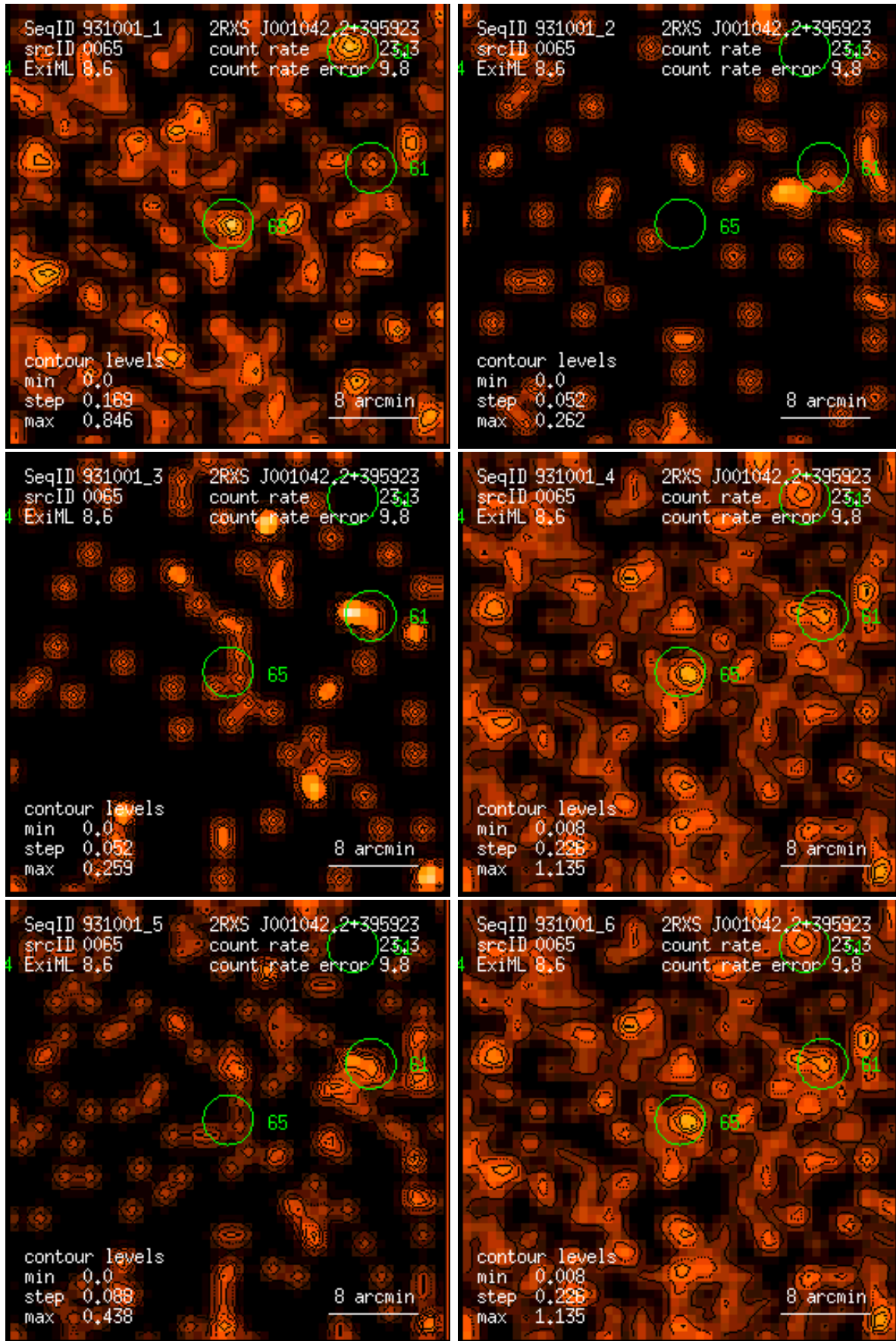
Figure 65: RASS 931001: detection 0065: band rate images, Gaussian filter: (1) PSPC channels 11 – 41, (2) 52 – 90, (3) 91 – 201, (4) 11 – 235, (5) 52 – 201, (6) 11 – 201. Broad band rates in counts/ks. Band rate contour levels in counts/ks/arcmin 2 .
