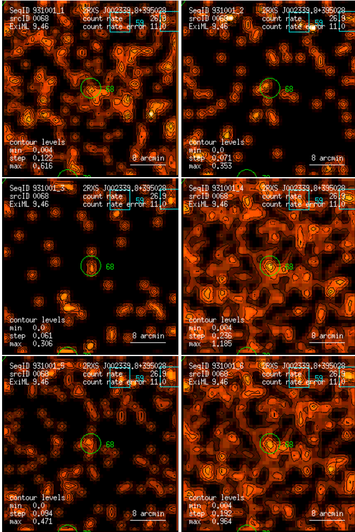
Figure 68: RASS 931001: detection 0068: band rate images, Gaussian filter: (1) PSPC channels 11 – 41, (2) 52 – 90, (3) 91 – 201, (4) 11 – 235, (5) 52 – 201, (6) 11 – 201. Broad band rates in counts/ks. Band rate contour levels in counts/ks/arcmin 2 .
