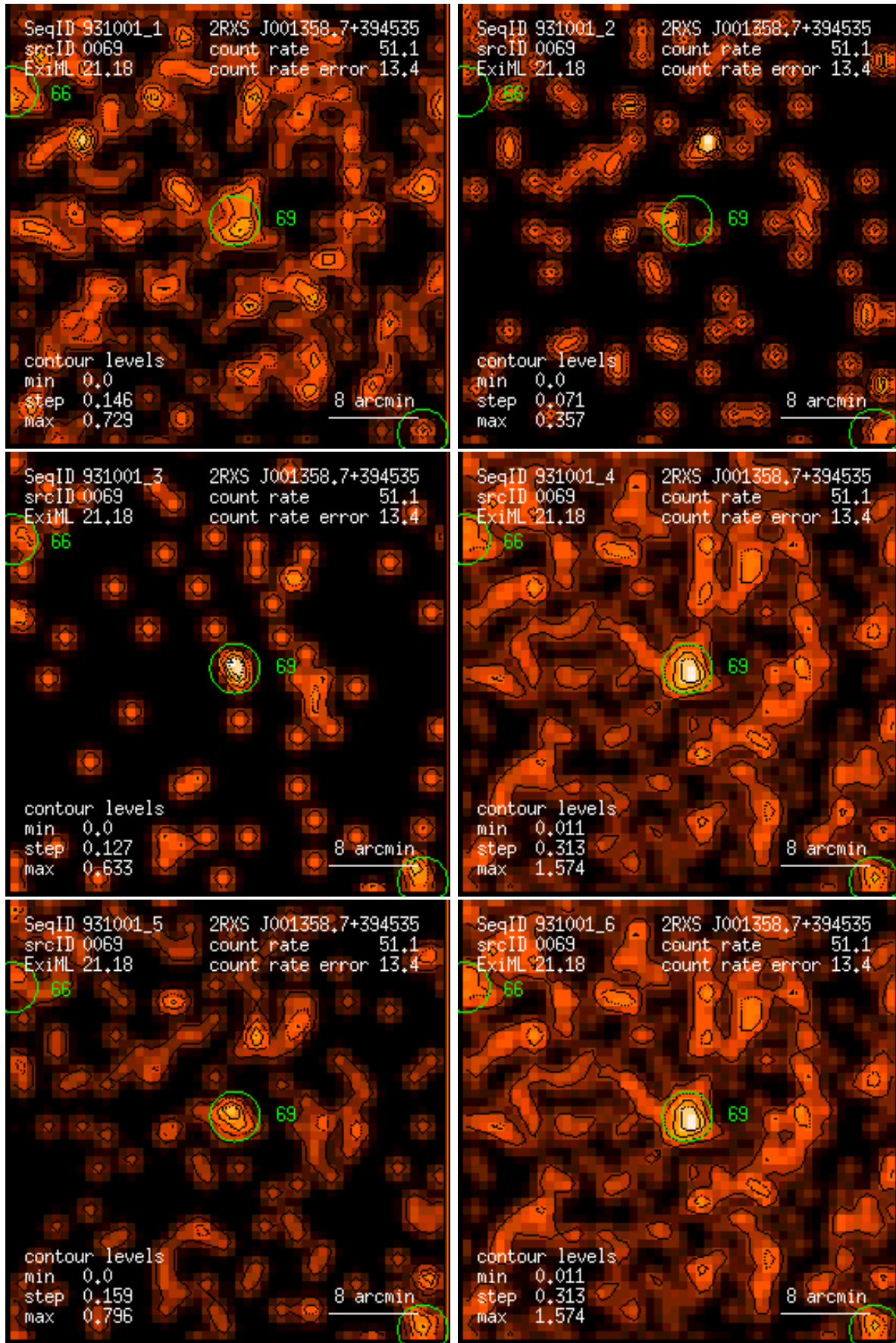
Figure 69: RASS 931001: detection 0069: band rate images, Gaussian filter: (1) PSPC channels 11 – 41, (2) 52 – 90, (3) 91 – 201, (4) 11 – 235, (5) 52 – 201, (6) 11 – 201. Broad band rates in counts/ks. Band rate contour levels in counts/ks/arcmin 2 .
