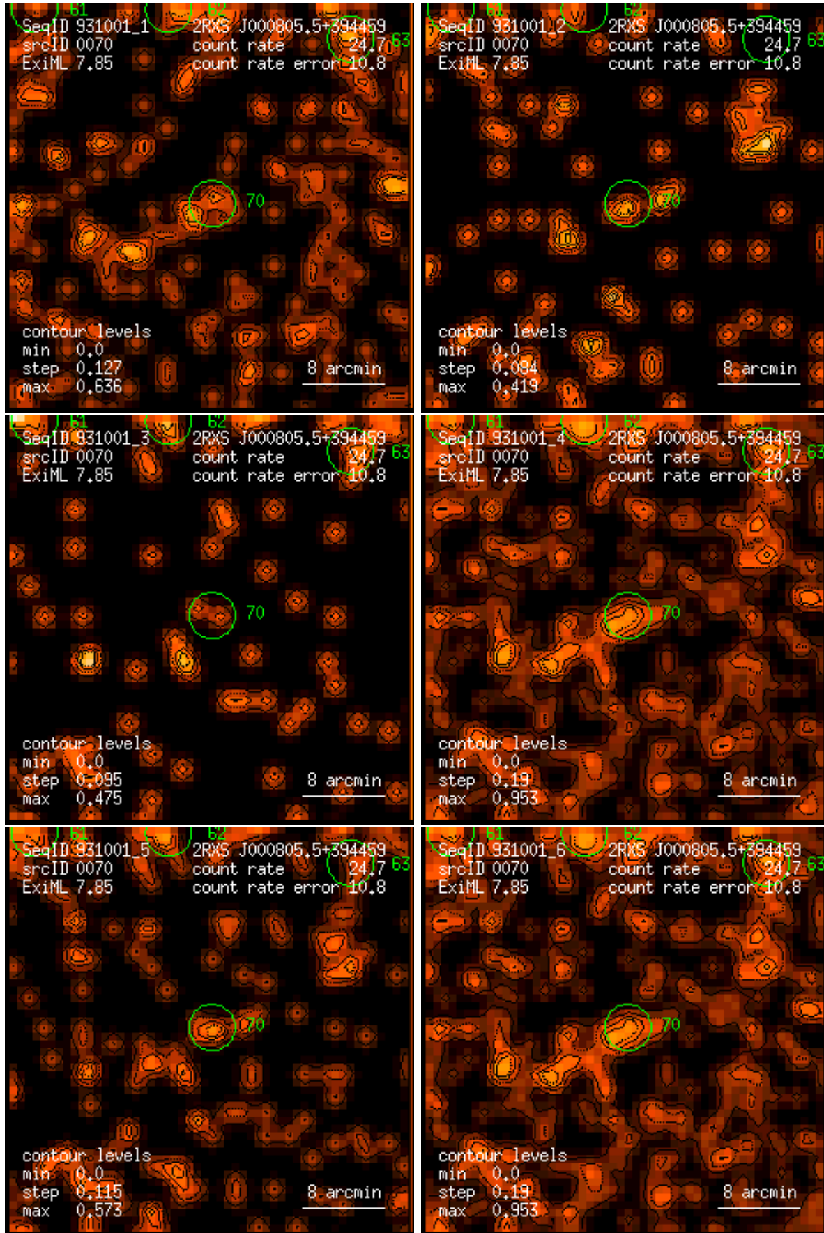
Figure 70: RASS 931001: detection 0070: band rate images, Gaussian filter: (1) PSPC channels 11 – 41, (2) 52 – 90, (3) 91 – 201, (4) 11 – 235, (5) 52 – 201, (6) 11 – 201. Broad band rates in counts/ks. Band rate contour levels in counts/ks/arcmin 2 .
