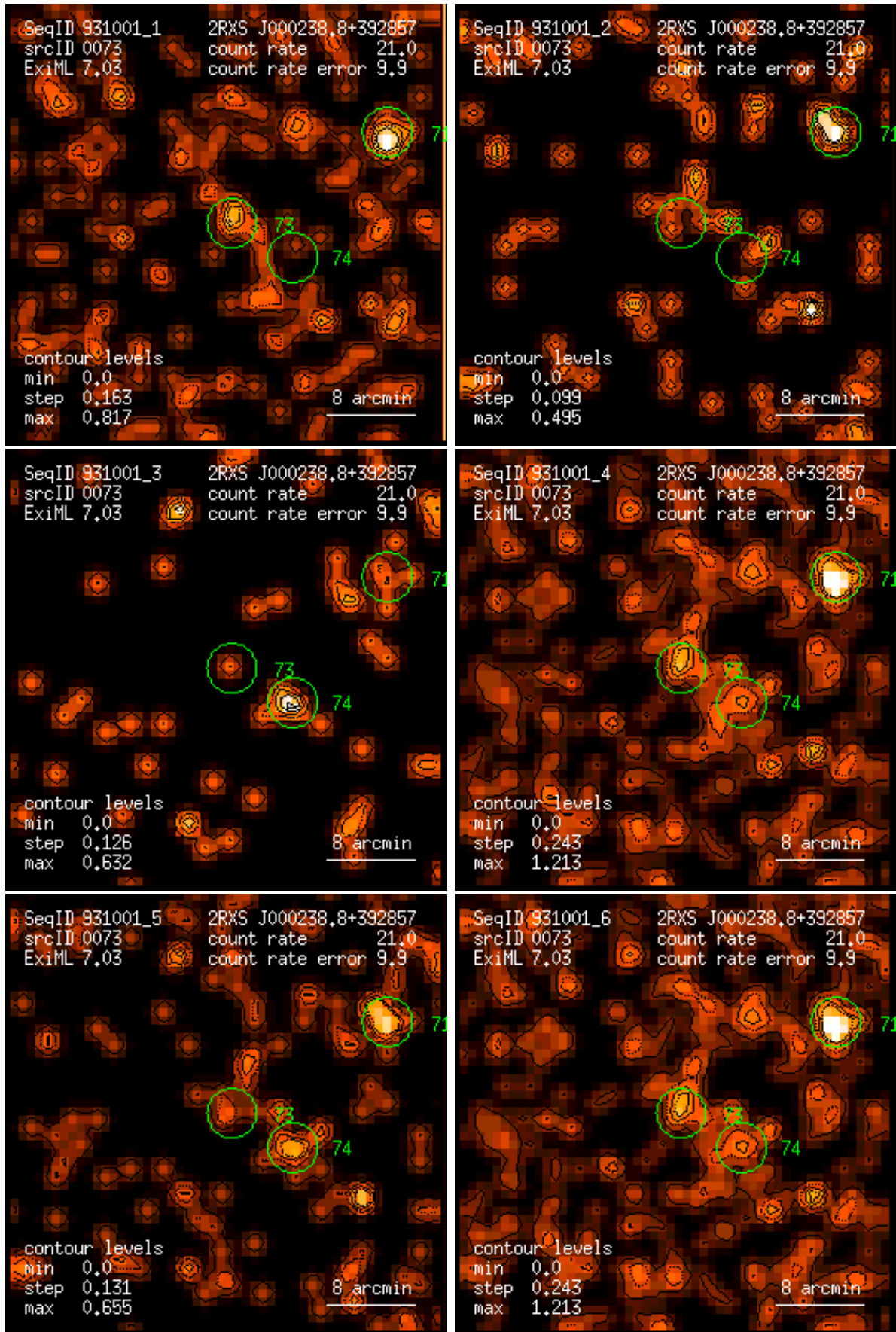
Figure 73: RASS 931001: detection 0073: band rate images, Gaussian filter: (1) PSPC channels 11 – 41, (2) 52 – 90, (3) 91 – 201, (4) 11 – 235, (5) 52 – 201, (6) 11 – 201. Broad band rates in counts/ks. Band rate contour levels in counts/ks/arcmin 2 .
