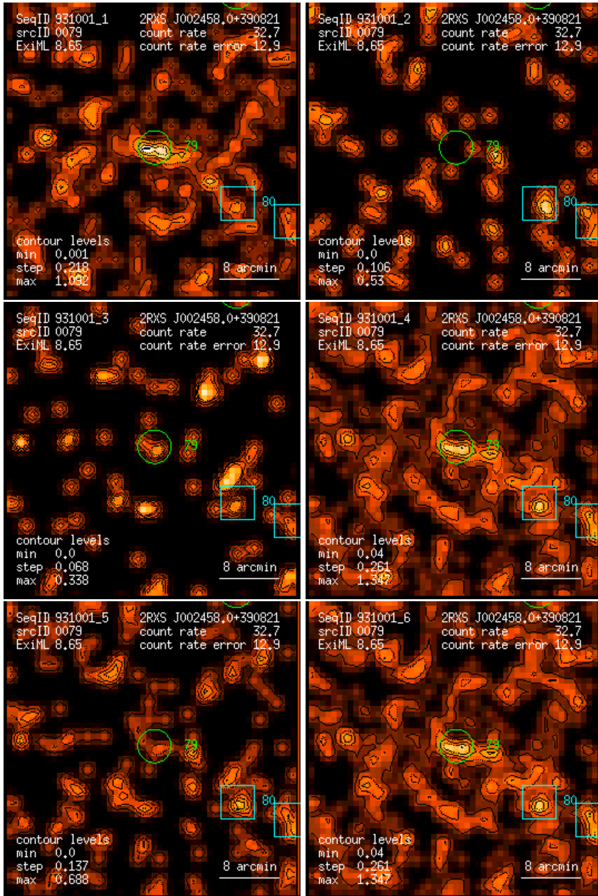
Figure 79: RASS 931001: detection 0079: band rate images, Gaussian filter: (1) PSPC channels 11 – 41, (2) 52 – 90, (3) 91 – 201, (4) 11 – 235, (5) 52 – 201, (6) 11 – 201. Broad band rates in counts/ks. Band rate contour levels in counts/ks/arcmin 2 .
