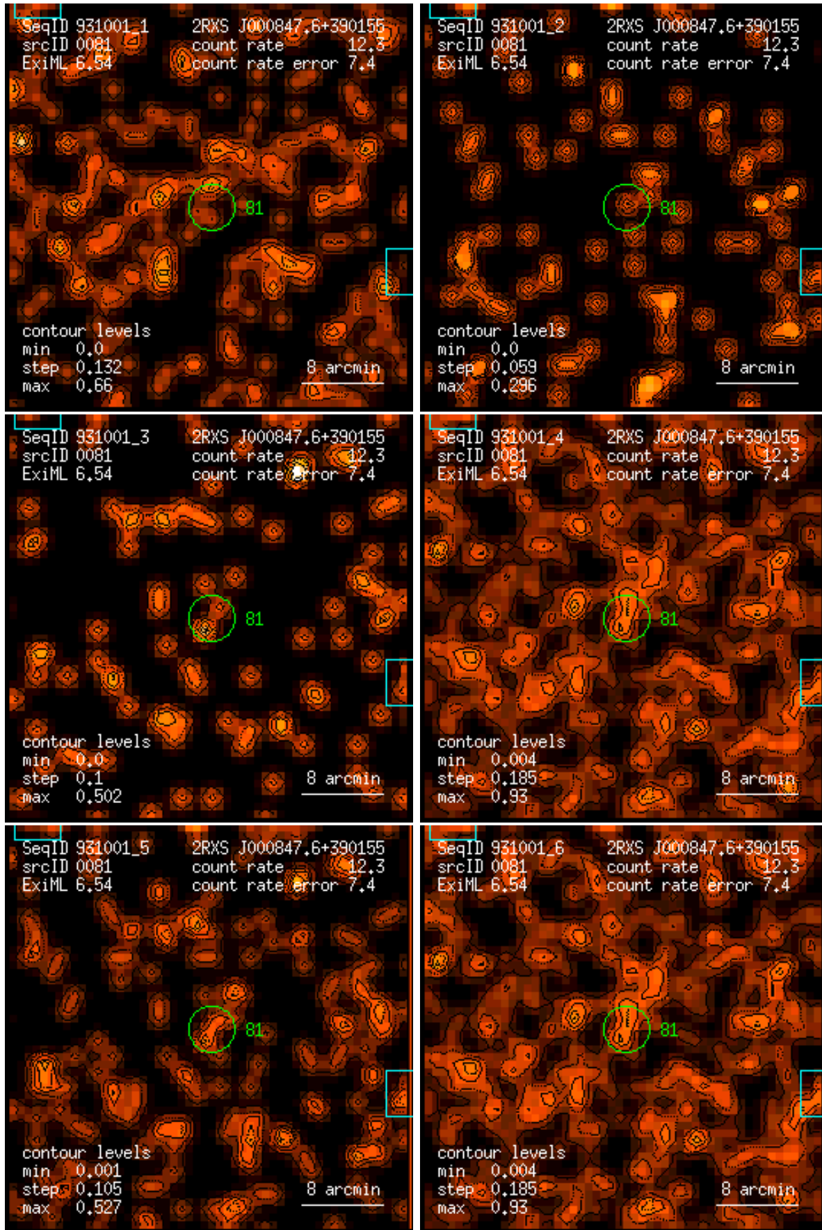
Figure 81: RASS 931001: detection 0081: band rate images, Gaussian filter: (1) PSPC channels 11 – 41, (2) 52 – 90, (3) 91 – 201, (4) 11 – 235, (5) 52 – 201, (6) 11 – 201. Broad band rates in counts/ks. Band rate contour levels in counts/ks/arcmin 2 .
